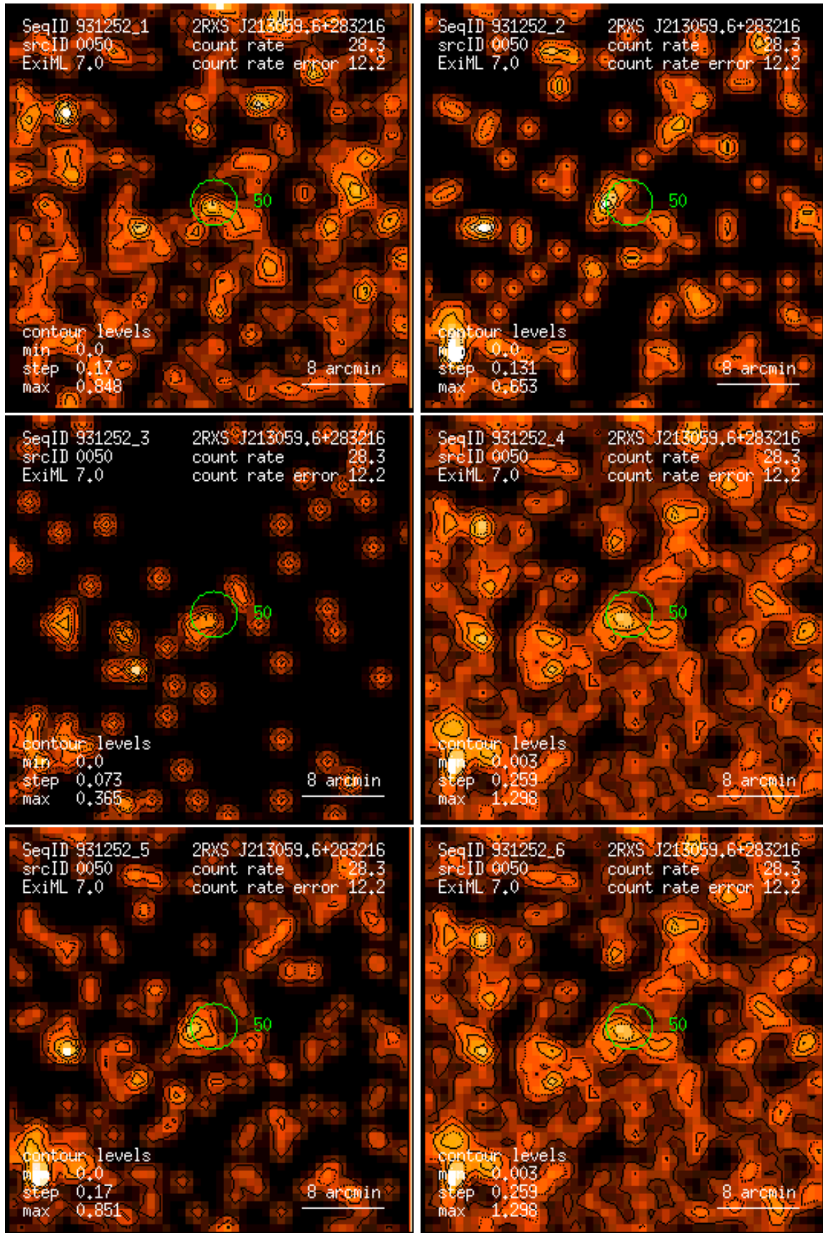
Figure 50: RASS 931252: detection 0050: band rate images, Gaussian filter: (1) PSPC channels 11 – 41, (2) 52 – 90, (3) 91 – 201, (4) 11 – 235, (5) 52 – 201, (6) 11 – 201. Broad band rates in counts/ks. Band rate contour levels in counts/ks/arcmin 2 .
