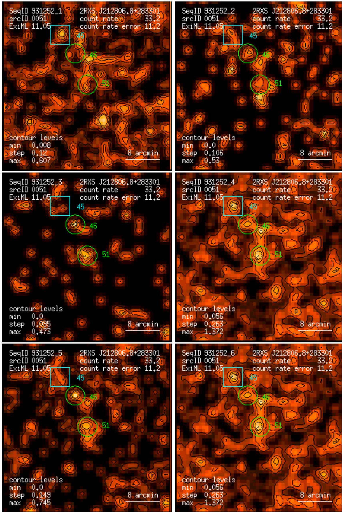
Figure 51: RASS 931252: detection 0051: band rate images, Gaussian filter: (1) PSPC channels 11 – 41, (2) 52 – 90, (3) 91 – 201, (4) 11 – 235, (5) 52 – 201, (6) 11 – 201. Broad band rates in counts/ks. Band rate contour levels in counts/ks/arcmin 2 .
