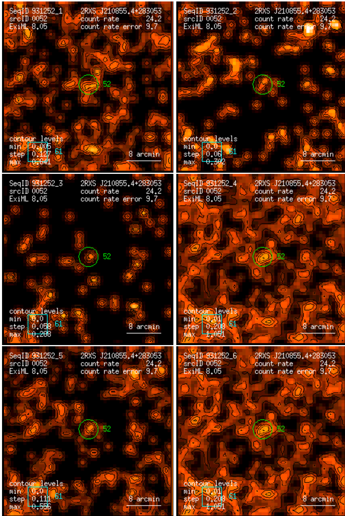
Figure 52: RASS 931252: detection 0052: band rate images, Gaussian filter: (1) PSPC channels 11 – 41, (2) 52 – 90, (3) 91 – 201, (4) 11 – 235, (5) 52 – 201, (6) 11 – 201. Broad band rates in counts/ks. Band rate contour levels in counts/ks/arcmin 2 .
