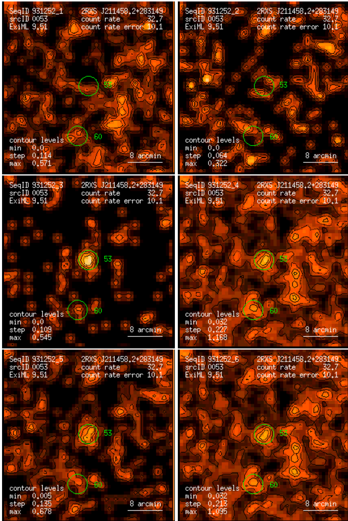
Figure 53: RASS 931252: detection 0053: band rate images, Gaussian filter: (1) PSPC channels 11 – 41, (2) 52 – 90, (3) 91 – 201, (4) 11 – 235, (5) 52 – 201, (6) 11 – 201. Broad band rates in counts/ks. Band rate contour levels in counts/ks/arcmin 2 .
