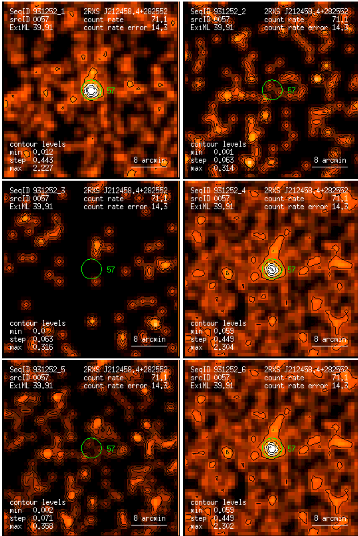
Figure 57: RASS 931252: detection 0057: band rate images, Gaussian filter: (1) PSPC channels 11 – 41, (2) 52 – 90, (3) 91 – 201, (4) 11 – 235, (5) 52 – 201, (6) 11 – 201. Broad band rates in counts/ks. Band rate contour levels in counts/ks/arcmin 2 .
