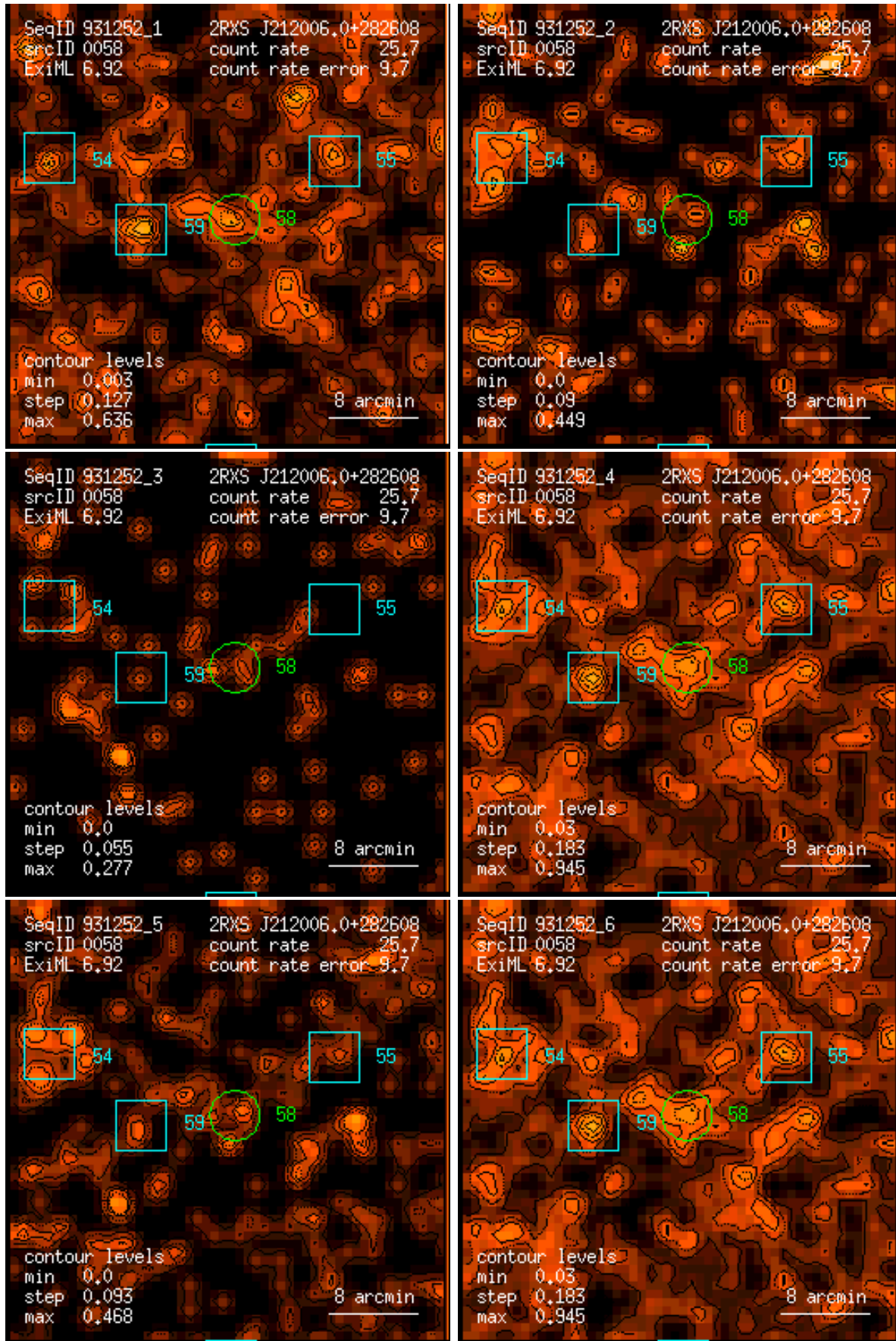
Figure 58: RASS 931252: detection 0058: band rate images, Gaussian filter: (1) PSPC channels 11 – 41, (2) 52 – 90, (3) 91 – 201, (4) 11 – 235, (5) 52 – 201, (6) 11 – 201. Broad band rates in counts/ks. Band rate contour levels in counts/ks/arcmin 2 .
