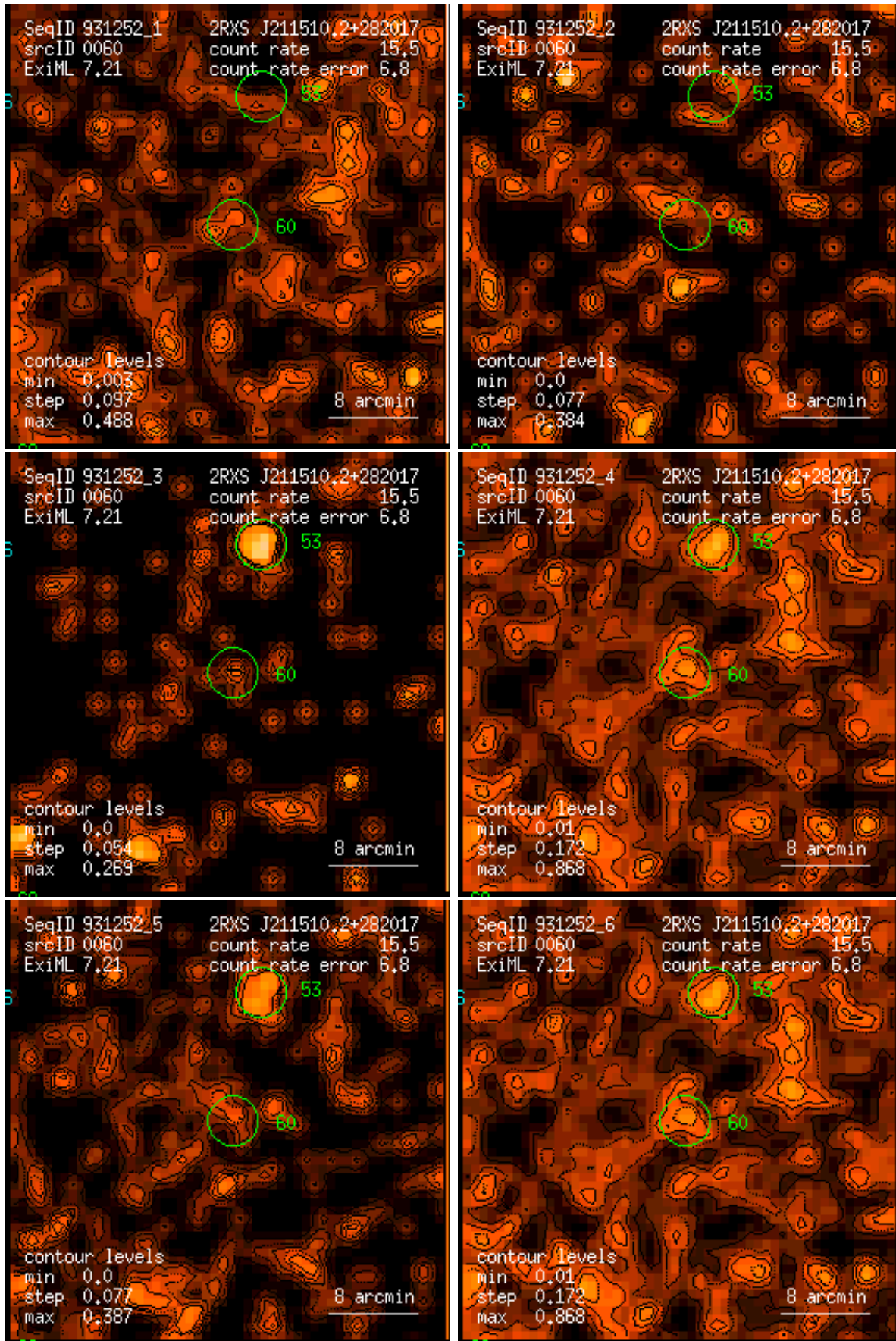
Figure 60: RASS 931252: detection 0060: band rate images, Gaussian filter: (1) PSPC channels 11 – 41, (2) 52 – 90, (3) 91 – 201, (4) 11 – 235, (5) 52 – 201, (6) 11 – 201. Broad band rates in counts/ks. Band rate contour levels in counts/ks/arcmin 2 .
