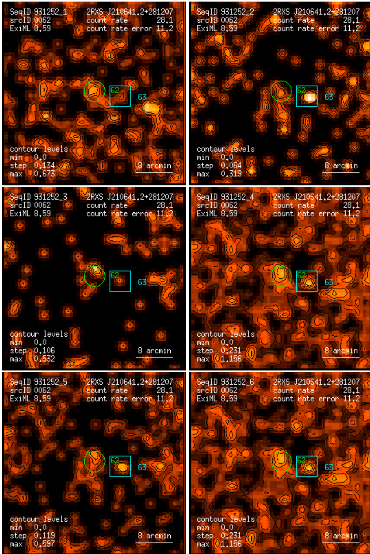
Figure 62: RASS 931252: detection 0062: band rate images, Gaussian filter: (1) PSPC channels 11 – 41, (2) 52 – 90, (3) 91 – 201, (4) 11 – 235, (5) 52 – 201, (6) 11 – 201. Broad band rates in counts/ks. Band rate contour levels in counts/ks/arcmin 2 .
