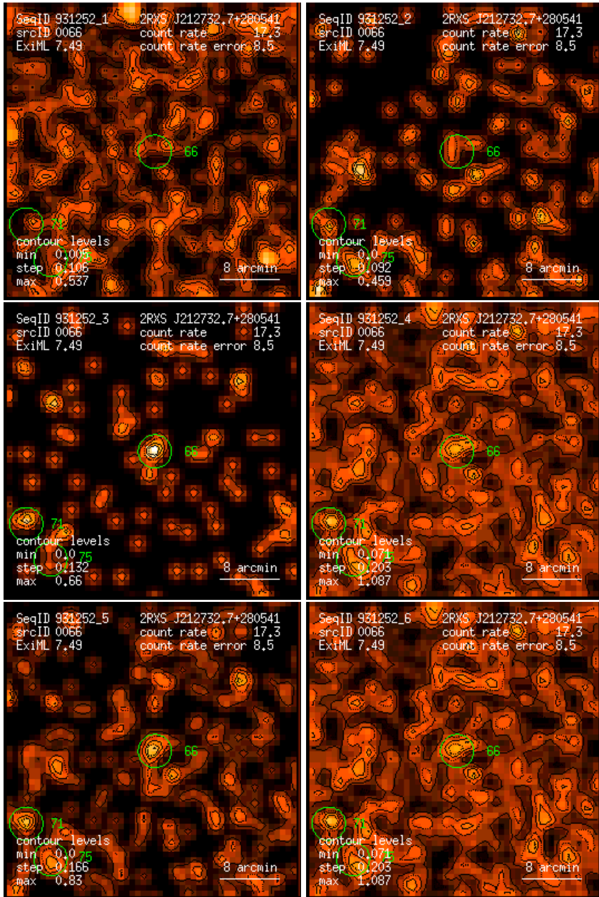
Figure 66: RASS 931252: detection 0066: band rate images, Gaussian filter: (1) PSPC channels 11 – 41, (2) 52 – 90, (3) 91 – 201, (4) 11 – 235, (5) 52 – 201, (6) 11 – 201. Broad band rates in counts/ks. Band rate contour levels in counts/ks/arcmin 2 .
