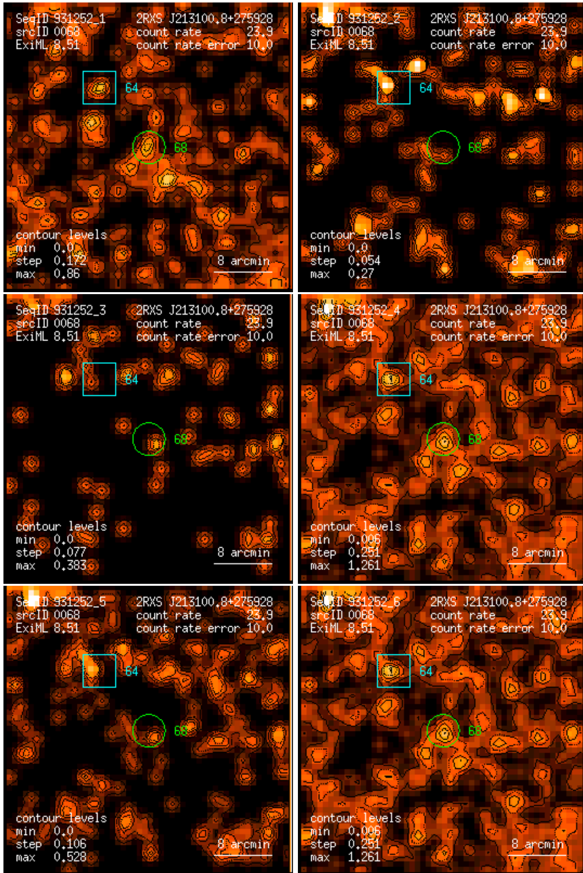
Figure 68: RASS 931252: detection 0068: band rate images, Gaussian filter: (1) PSPC channels 11 – 41, (2) 52 – 90, (3) 91 – 201, (4) 11 – 235, (5) 52 – 201, (6) 11 – 201. Broad band rates in counts/ks. Band rate contour levels in counts/ks/arcmin 2 .
