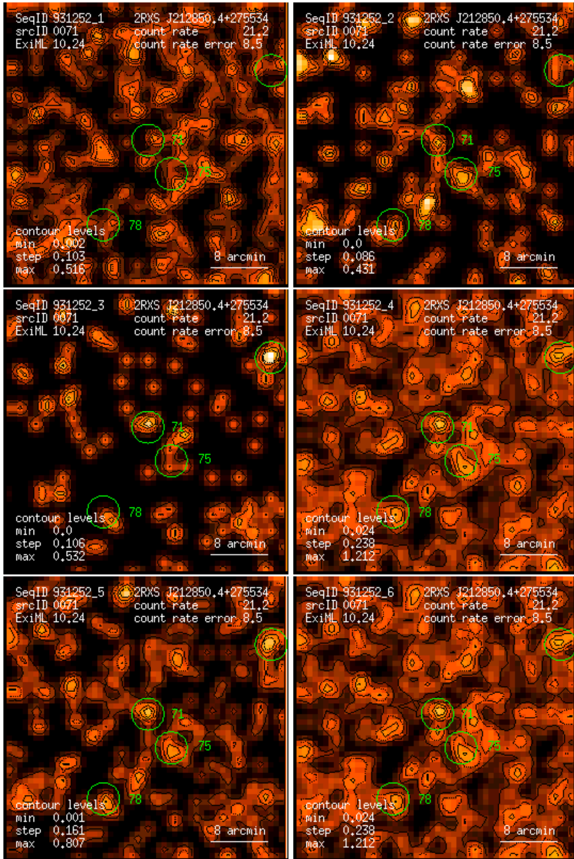
Figure 71: RASS 931252: detection 0071: band rate images, Gaussian filter: (1) PSPC channels 11 – 41, (2) 52 – 90, (3) 91 – 201, (4) 11 – 235, (5) 52 – 201, (6) 11 – 201. Broad band rates in counts/ks. Band rate contour levels in counts/ks/arcmin 2 .
