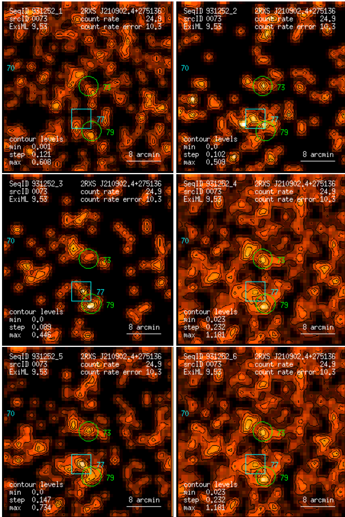
Figure 73: RASS 931252: detection 0073: band rate images, Gaussian filter: (1) PSPC channels 11 – 41, (2) 52 – 90, (3) 91 – 201, (4) 11 – 235, (5) 52 – 201, (6) 11 – 201. Broad band rates in counts/ks. Band rate contour levels in counts/ks/arcmin 2 .
