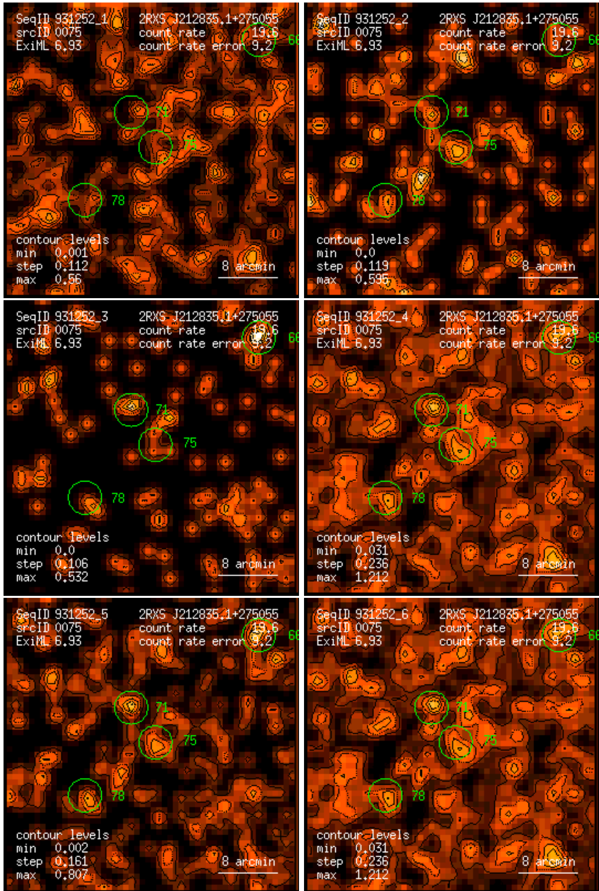
Figure 75: RASS 931252: detection 0075: band rate images, Gaussian filter: (1) PSPC channels 11 – 41, (2) 52 – 90, (3) 91 – 201, (4) 11 – 235, (5) 52 – 201, (6) 11 – 201. Broad band rates in counts/ks. Band rate contour levels in counts/ks/arcmin 2 .
