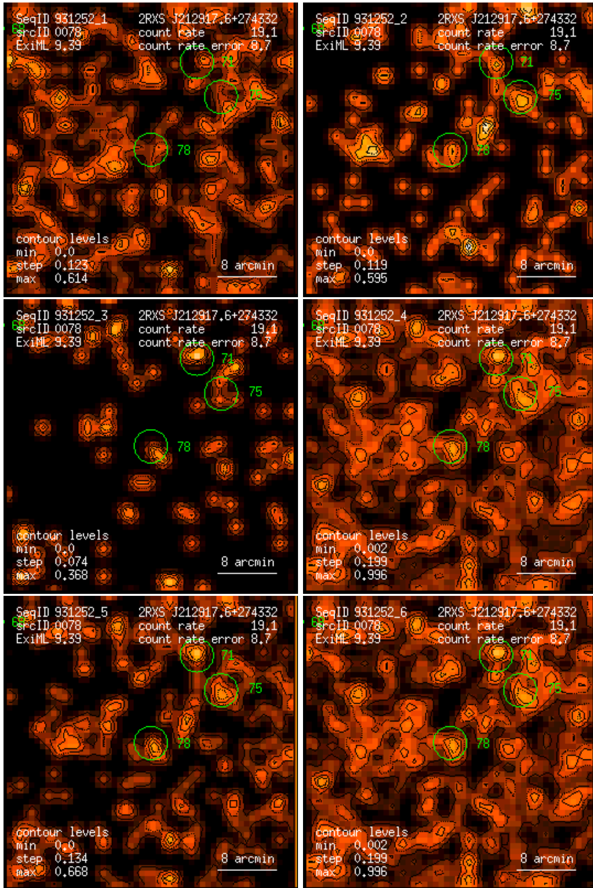
Figure 78: RASS 931252: detection 0078: band rate images, Gaussian filter: (1) PSPC channels 11 – 41, (2) 52 – 90, (3) 91 – 201, (4) 11 – 235, (5) 52 – 201, (6) 11 – 201. Broad band rates in counts/ks. Band rate contour levels in counts/ks/arcmin 2 .
