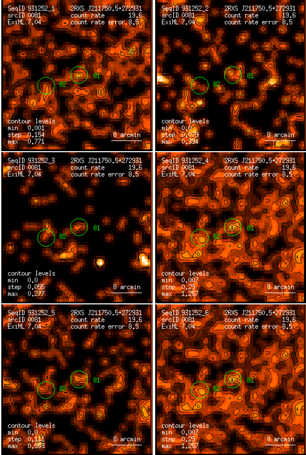
Figure 81: RASS 931252: detection 0081: band rate images, Gaussian filter: (1) PSPC channels 11 – 41, (2) 52 – 90, (3) 91 – 201, (4) 11 – 235, (5) 52 – 201, (6) 11 – 201. Broad band rates in counts/ks. Band rate contour levels in counts/ks/arcmin 2 .
