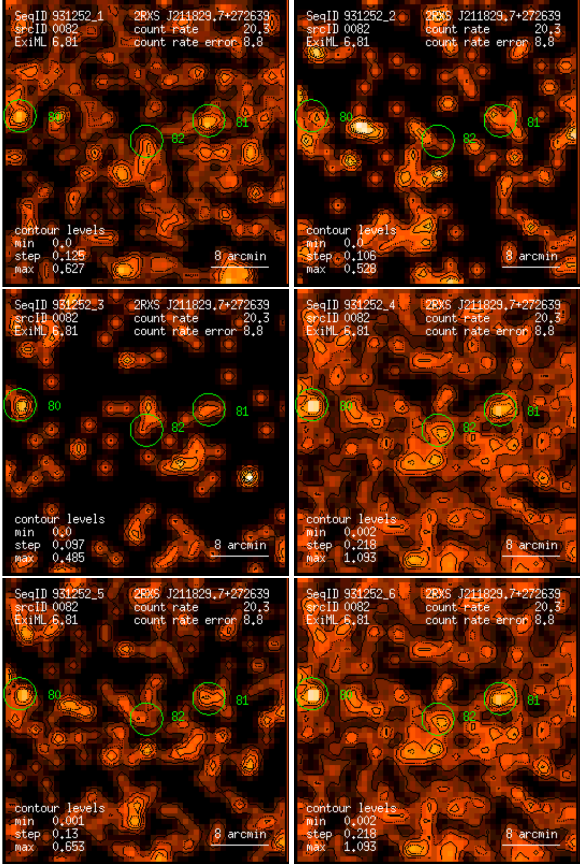
Figure 82: RASS 931252: detection 0082: band rate images, Gaussian filter: (1) PSPC channels 11 – 41, (2) 52 – 90, (3) 91 – 201, (4) 11 – 235, (5) 52 – 201, (6) 11 – 201. Broad band rates in counts/ks. Band rate contour levels in counts/ks/arcmin 2 .
