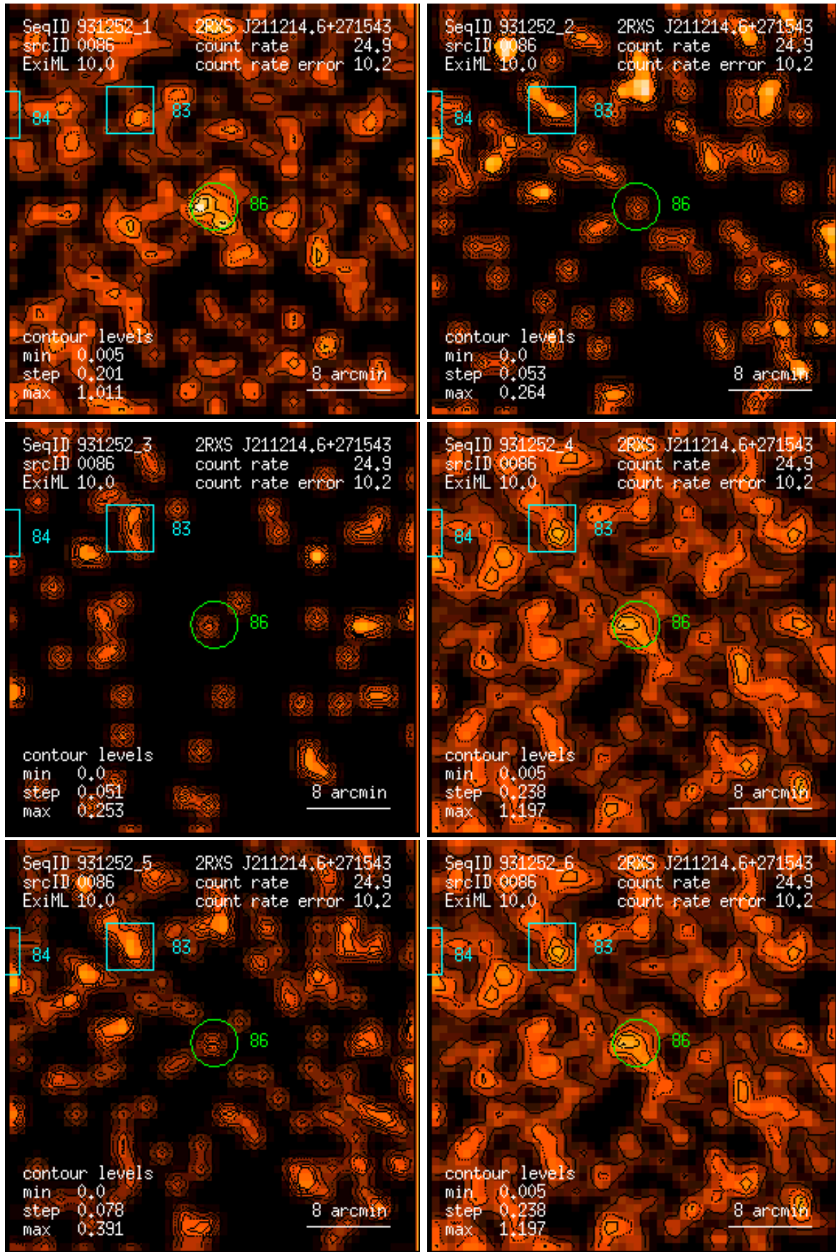
Figure 86: RASS 931252: detection 0086: band rate images, Gaussian filter: (1) PSPC channels 11 – 41, (2) 52 – 90, (3) 91 – 201, (4) 11 – 235, (5) 52 – 201, (6) 11 – 201. Broad band rates in counts/ks. Band rate contour levels in counts/ks/arcmin 2 .
