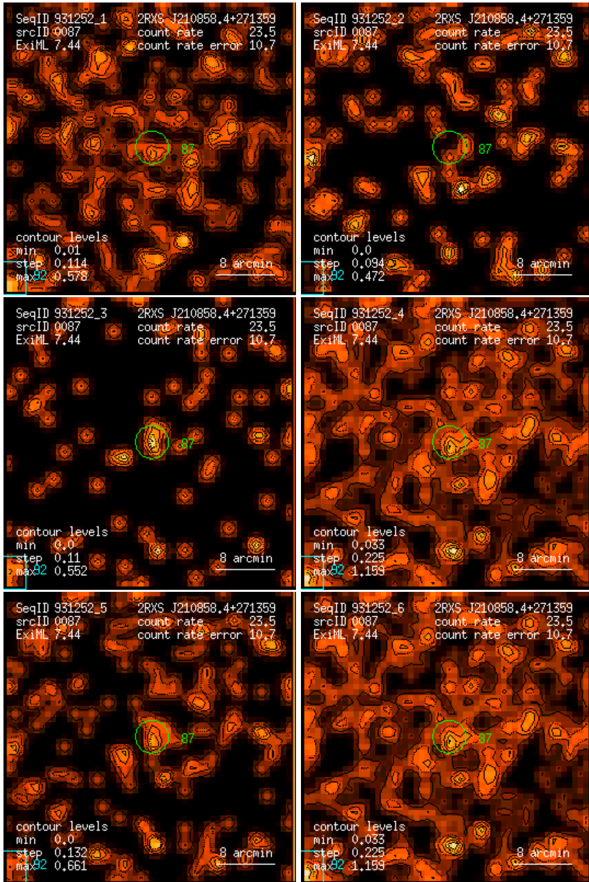
Figure 87: RASS 931252: detection 0087: band rate images, Gaussian filter: (1) PSPC channels 11 – 41, (2) 52 – 90, (3) 91 – 201, (4) 11 – 235, (5) 52 – 201, (6) 11 – 201. Broad band rates in counts/ks. Band rate contour levels in counts/ks/arcmin 2 .
