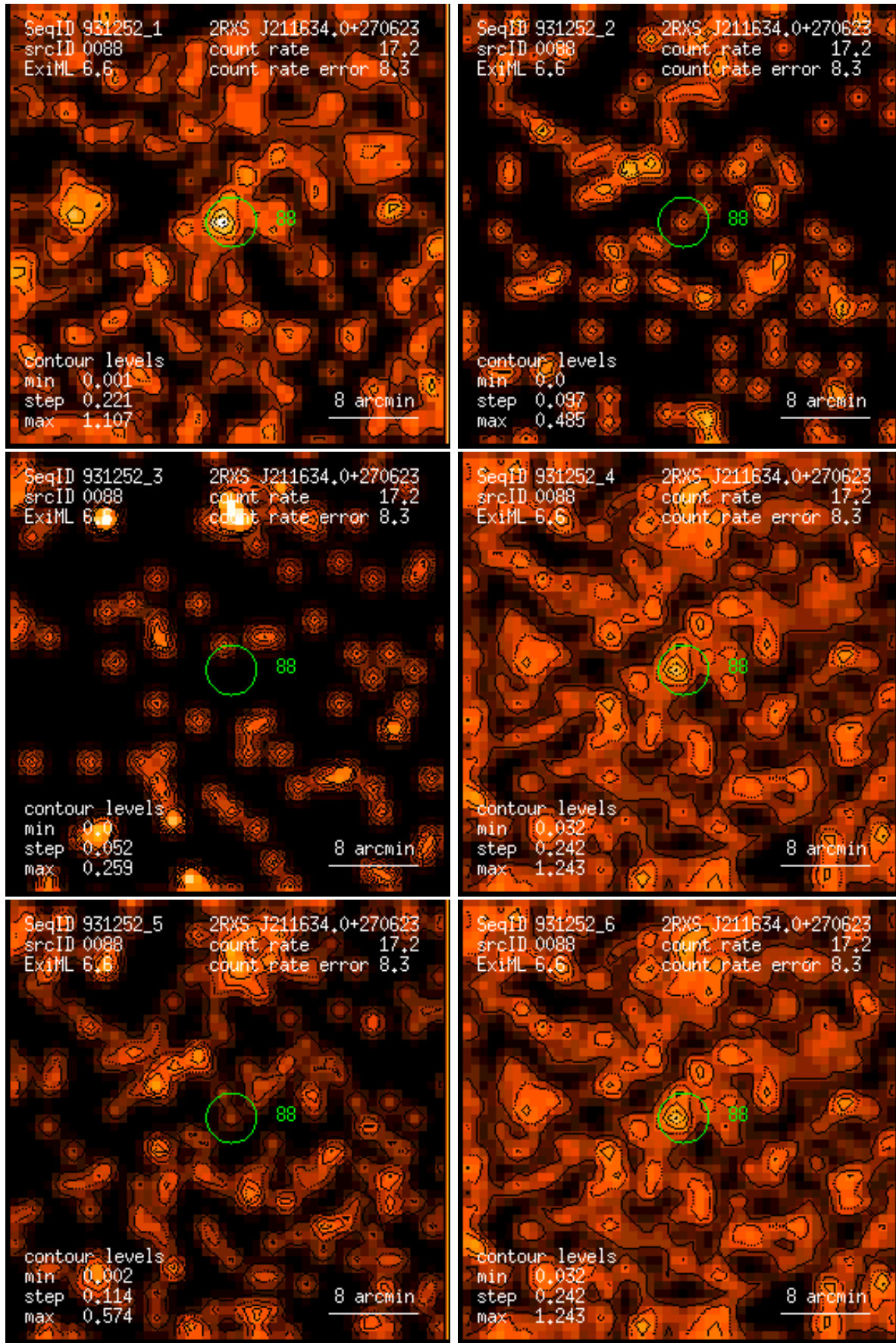
Figure 88: RASS 931252: detection 0088: band rate images, Gaussian filter: (1) PSPC channels 11 – 41, (2) 52 – 90, (3) 91 – 201, (4) 11 – 235, (5) 52 – 201, (6) 11 – 201. Broad band rates in counts/ks. Band rate contour levels in counts/ks/arcmin 2 .
