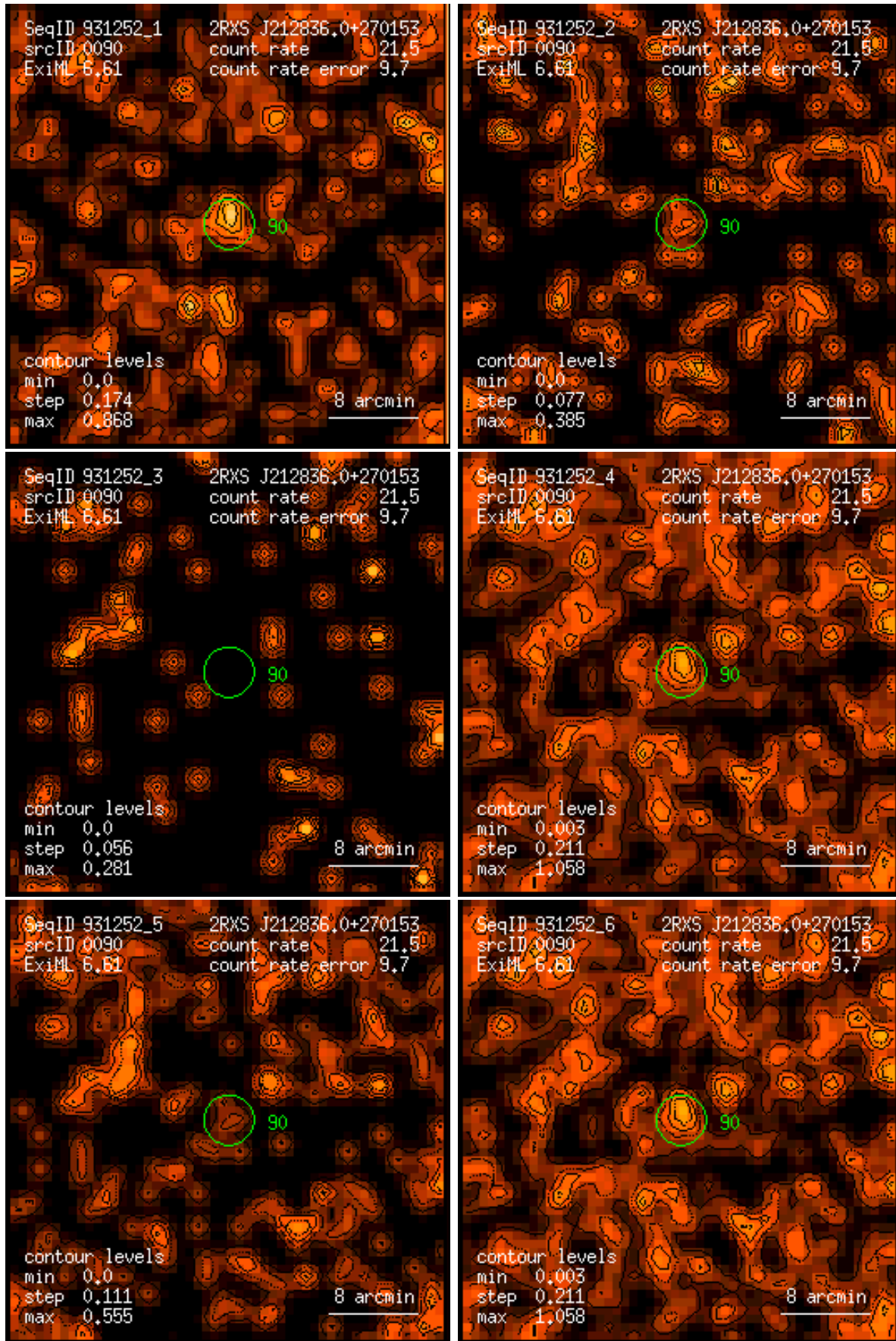
Figure 90: RASS 931252: detection 0090: band rate images, Gaussian filter: (1) PSPC channels 11 – 41, (2) 52 – 90, (3) 91 – 201, (4) 11 – 235, (5) 52 – 201, (6) 11 – 201. Broad band rates in counts/ks. Band rate contour levels in counts/ks/arcmin 2 .
