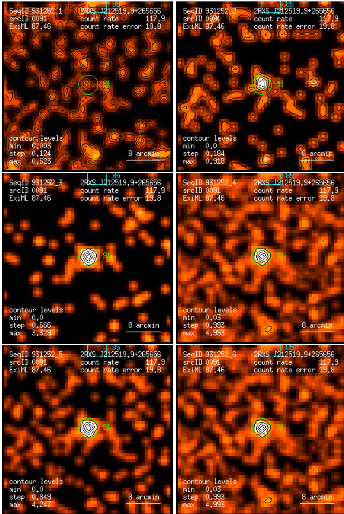
Figure 91: RASS 931252: detection 0091: band rate images, Gaussian filter: (1) PSPC channels 11 – 41, (2) 52 – 90, (3) 91 – 201, (4) 11 – 235, (5) 52 – 201, (6) 11 – 201. Broad band rates in counts/ks. Band rate contour levels in counts/ks/arcmin 2 .
