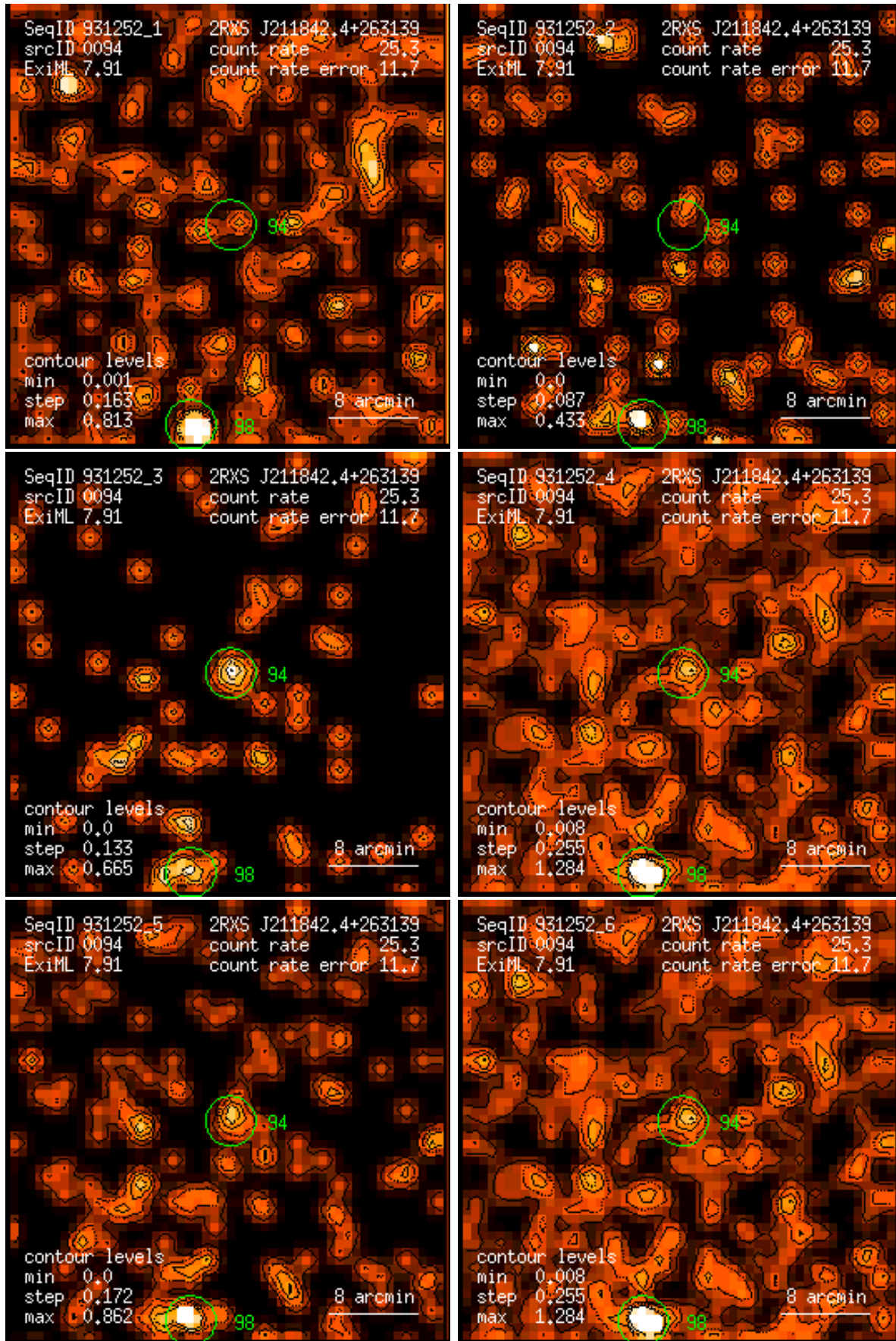
Figure 94: RASS 931252: detection 0094: band rate images, Gaussian filter: (1) PSPC channels 11 – 41, (2) 52 – 90, (3) 91 – 201, (4) 11 – 235, (5) 52 – 201, (6) 11 – 201. Broad band rates in counts/ks. Band rate contour levels in counts/ks/arcmin 2 .
