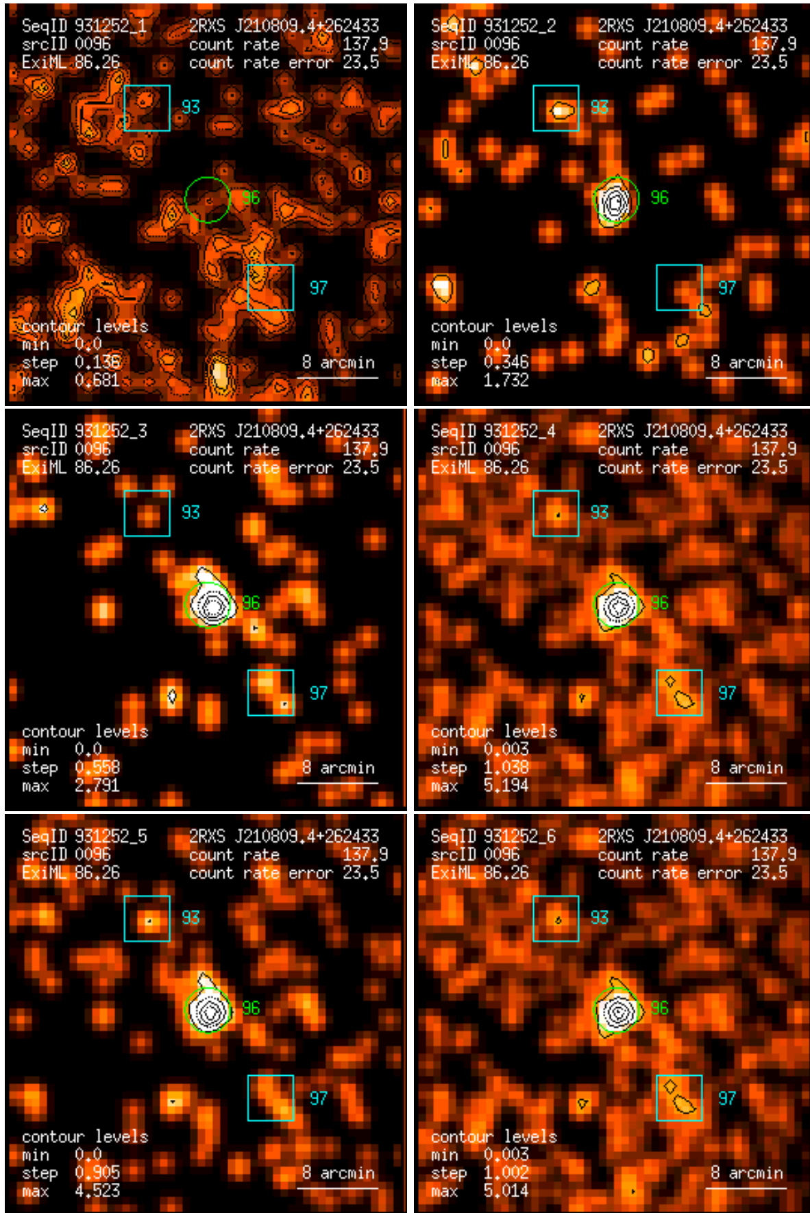
Figure 96: RASS 931252: detection 0096: band rate images, Gaussian filter: (1) PSPC channels 11 – 41, (2) 52 – 90, (3) 91 – 201, (4) 11 – 235, (5) 52 – 201, (6) 11 – 201. Broad band rates in counts/ks. Band rate contour levels in counts/ks/arcmin 2 .
