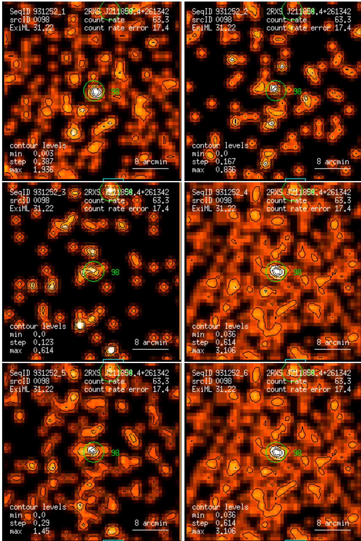
Figure 98: RASS 931252: detection 0098: band rate images, Gaussian filter: (1) PSPC channels 11 – 41, (2) 52 – 90, (3) 91 – 201, (4) 11 – 235, (5) 52 – 201, (6) 11 – 201. Broad band rates in counts/ks. Band rate contour levels in counts/ks/arcmin 2 .
