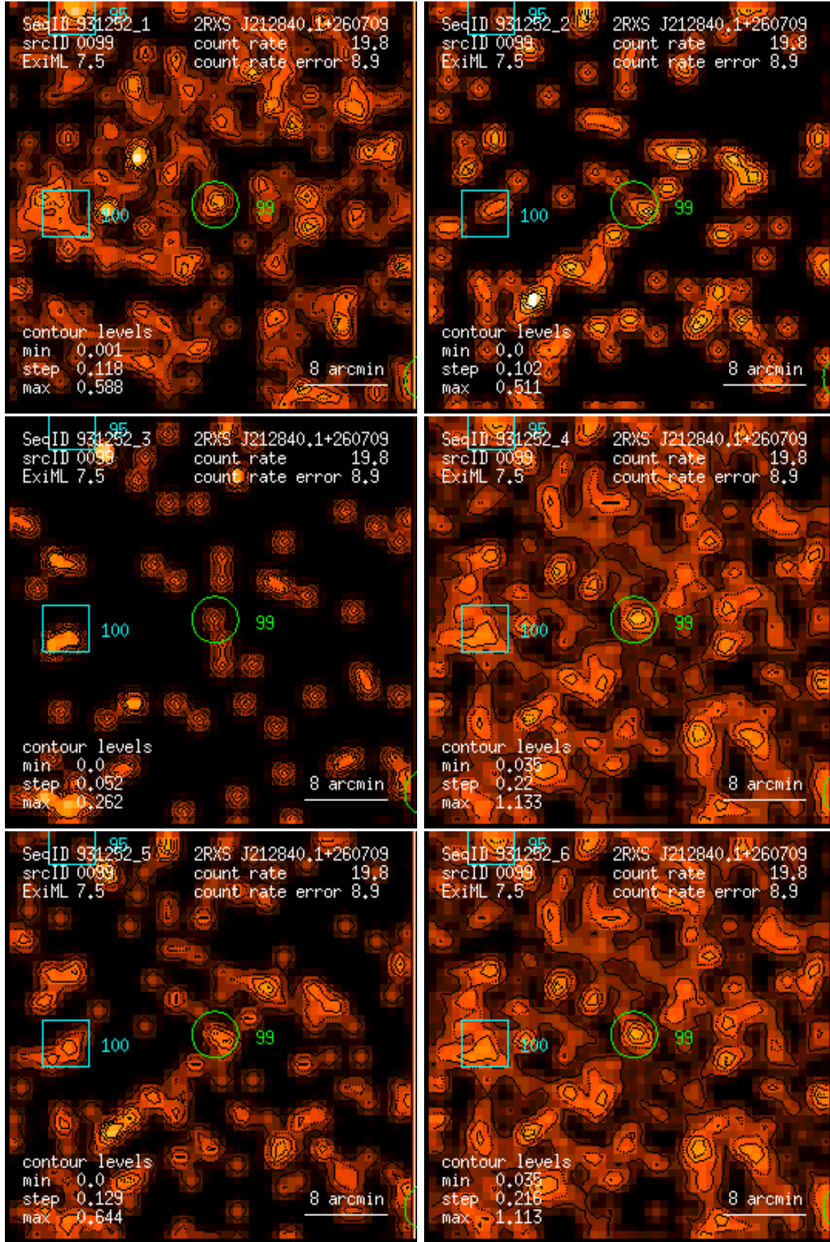
Figure 99: RASS 931252: detection 0099: band rate images, Gaussian filter: (1) PSPC channels 11 – 41, (2) 52 – 90, (3) 91 – 201, (4) 11 – 235, (5) 52 – 201, (6) 11 – 201. Broad band rates in counts/ks. Band rate contour levels in counts/ks/arcmin 2 .
