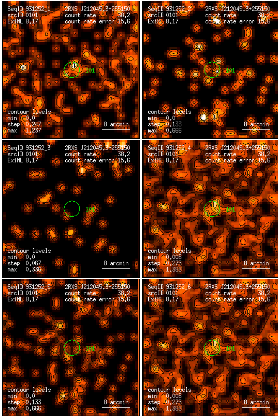
Figure 101: RASS 931252: detection 0101: band rate images, Gaussian filter: (1) PSPC channels 11 – 41, (2) 52 – 90, (3) 91 – 201, (4) 11 – 235, (5) 52 – 201, (6) 11 – 201. Broad band rates in counts/ks. Band rate contour levels in counts/ks/arcmin 2 .
