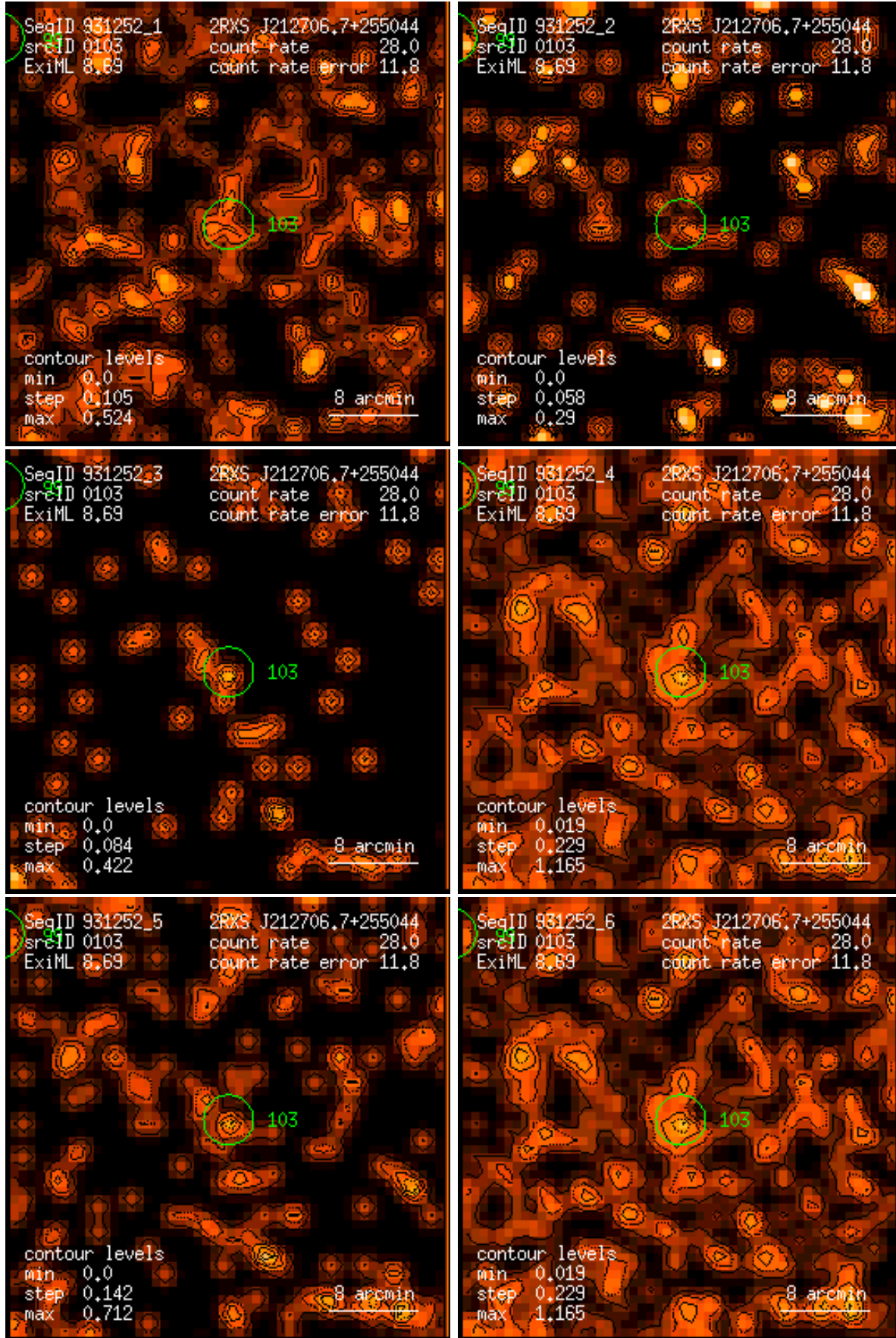
Figure 103: RASS 931252: detection 0103: band rate images, Gaussian filter: (1) PSPC channels 11 – 41, (2) 52 – 90, (3) 91 – 201, (4) 11 – 235, (5) 52 – 201, (6) 11 – 201. Broad band rates in counts/ks. Band rate contour levels in counts/ks/arcmin 2 .
