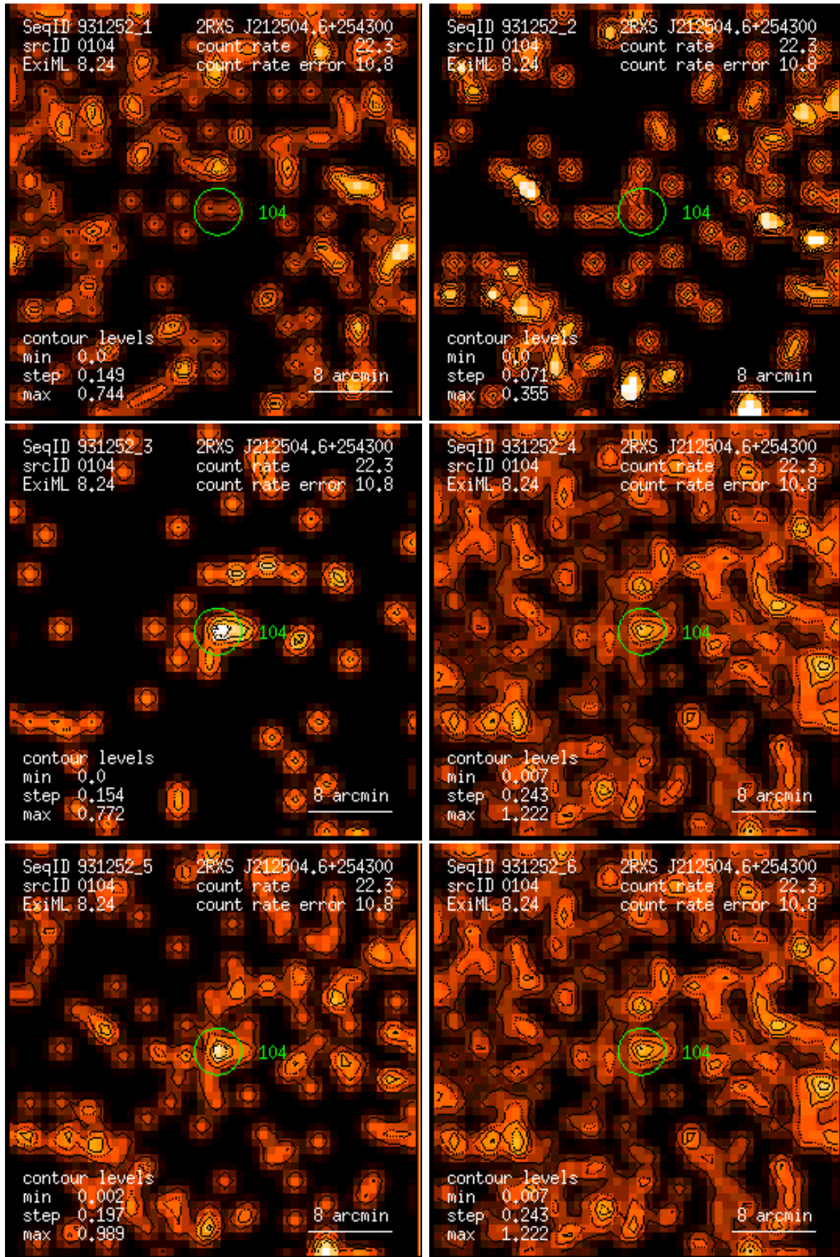
Figure 104: RASS 931252: detection 0104: band rate images, Gaussian filter: (1) PSPC channels 11 – 41, (2) 52 – 90, (3) 91 – 201, (4) 11 – 235, (5) 52 – 201, (6) 11 – 201. Broad band rates in counts/ks. Band rate contour levels in counts/ks/arcmin 2 .
