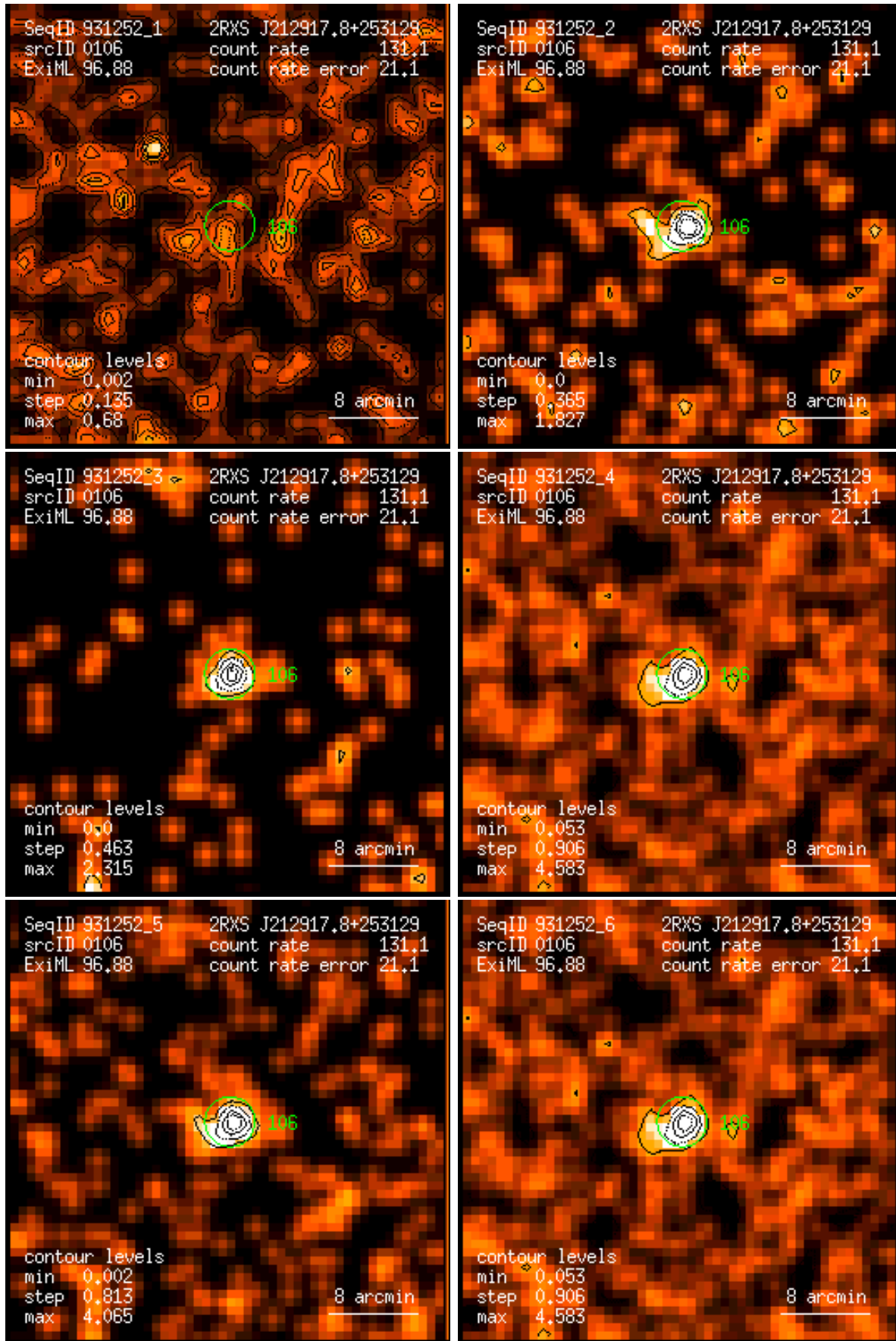
Figure 106: RASS 931252: detection 0106: band rate images, Gaussian filter: (1) PSPC channels 11 – 41, (2) 52 – 90, (3) 91 – 201, (4) 11 – 235, (5) 52 – 201, (6) 11 – 201. Broad band rates in counts/ks. Band rate contour levels in counts/ks/arcmin 2 .
