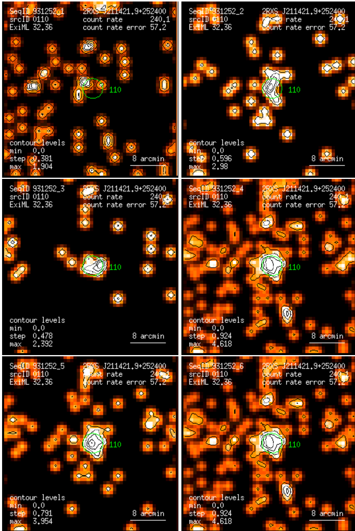
Figure 110: RASS 931252: detection 0110: band rate images, Gaussian filter: (1) PSPC channels 11 – 41, (2) 52 – 90, (3) 91 – 201, (4) 11 – 235, (5) 52 – 201, (6) 11 – 201. Broad band rates in counts/ks. Band rate contour levels in counts/ks/arcmin 2 .
