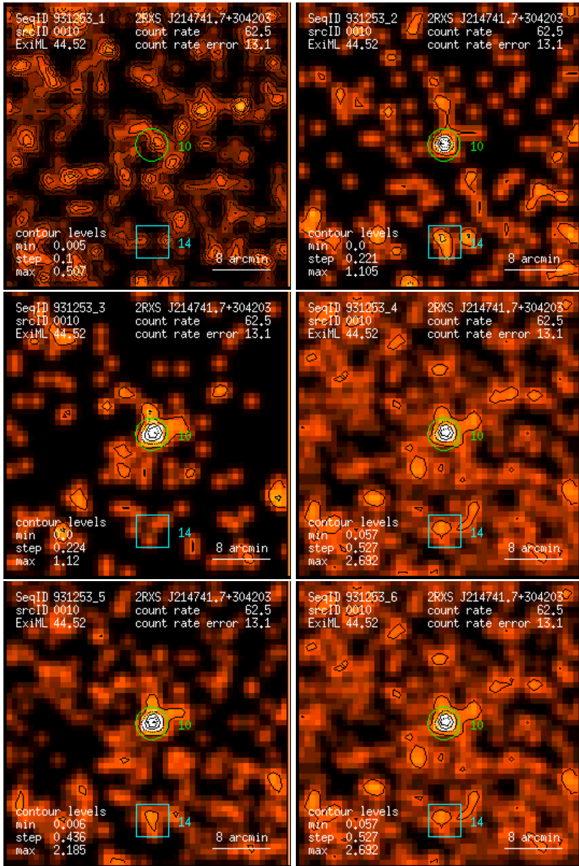
Figure 10: RASS 931253: detection 0010: band rate images, Gaussian filter: (1) PSPC channels 11 – 41, (2) 52 – 90, (3) 91 – 201, (4) 11 – 235, (5) 52 – 201, (6) 11 – 201. Broad band rates in counts/ks. Band rate contour levels in counts/ks/arcmin 2 .
