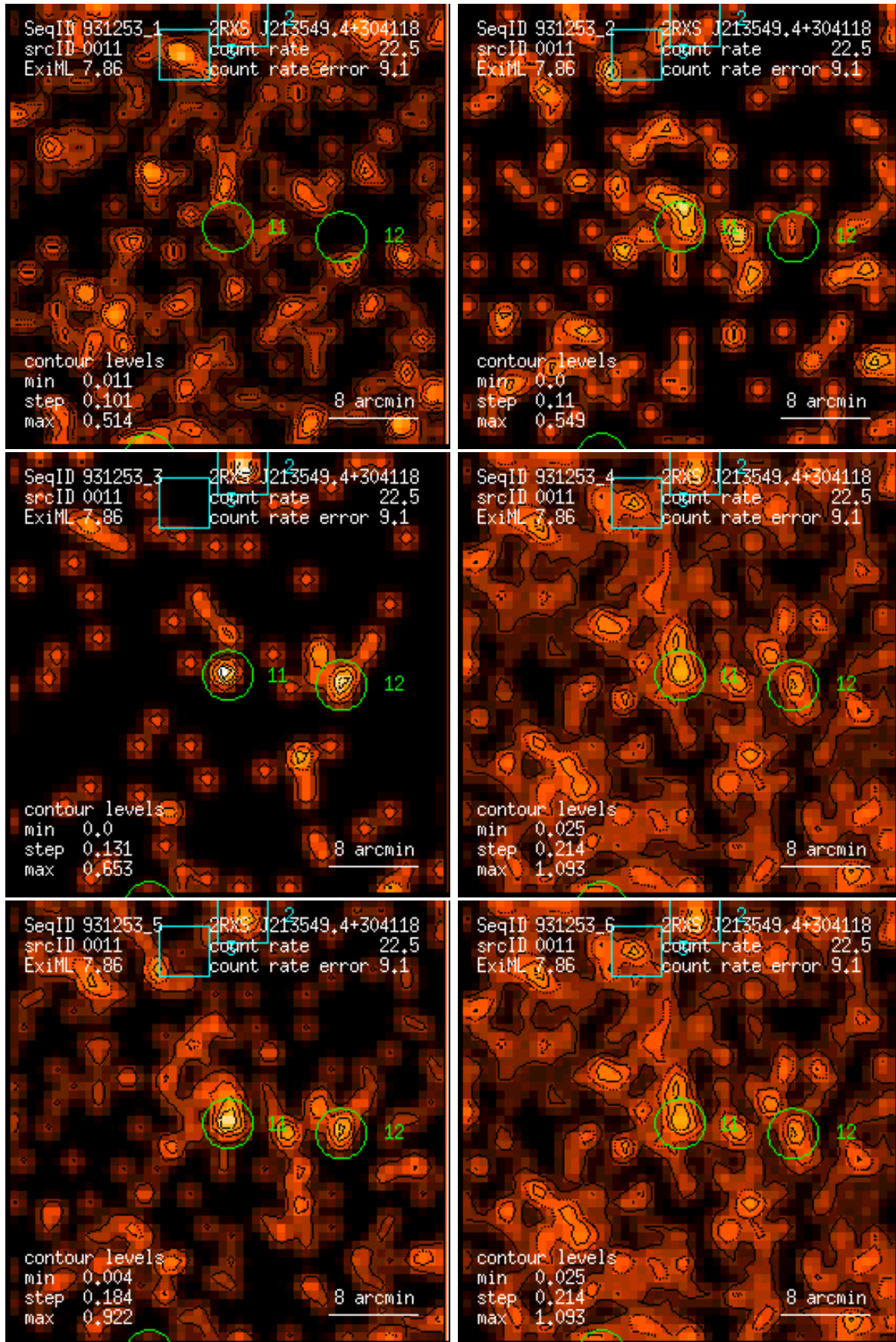
Figure 11: RASS 931253: detection 0011: band rate images, Gaussian filter: (1) PSPC channels 11 – 41, (2) 52 – 90, (3) 91 – 201, (4) 11 – 235, (5) 52 – 201, (6) 11 – 201. Broad band rates in counts/ks. Band rate contour levels in counts/ks/arcmin 2 .
