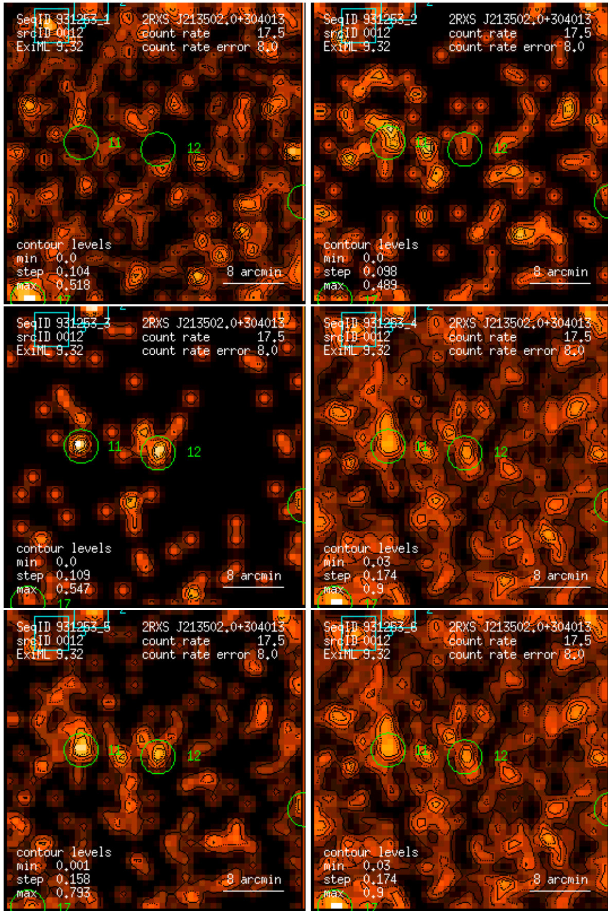
Figure 12: RASS 931253: detection 0012: band rate images, Gaussian filter: (1) PSPC channels 11 – 41, (2) 52 – 90, (3) 91 – 201, (4) 11 – 235, (5) 52 – 201, (6) 11 – 201. Broad band rates in counts/ks. Band rate contour levels in counts/ks/arcmin 2 .
