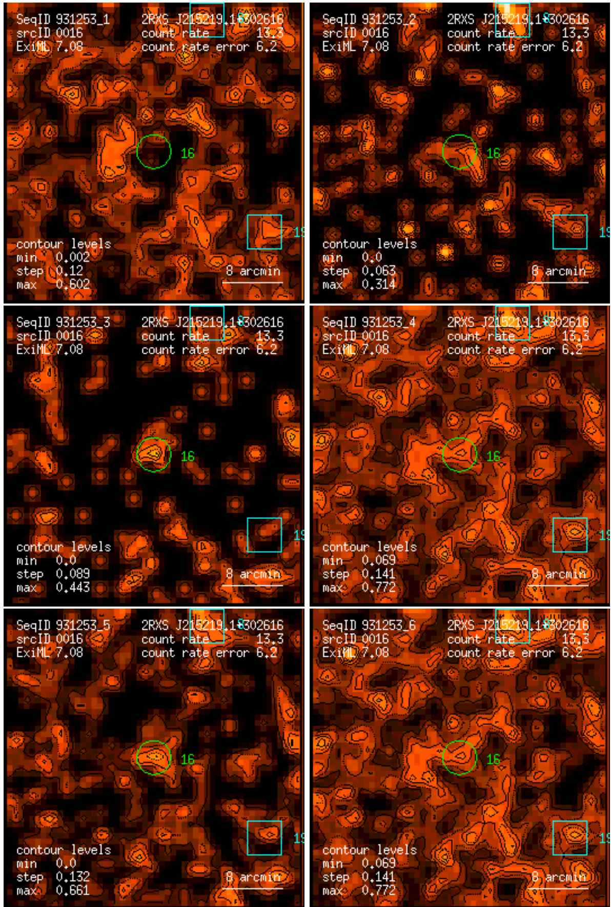
Figure 16: RASS 931253: detection 0016: band rate images, Gaussian filter: (1) PSPC channels 11 – 41, (2) 52 – 90, (3) 91 – 201, (4) 11 – 235, (5) 52 – 201, (6) 11 – 201. Broad band rates in counts/ks. Band rate contour levels in counts/ks/arcmin 2 .
