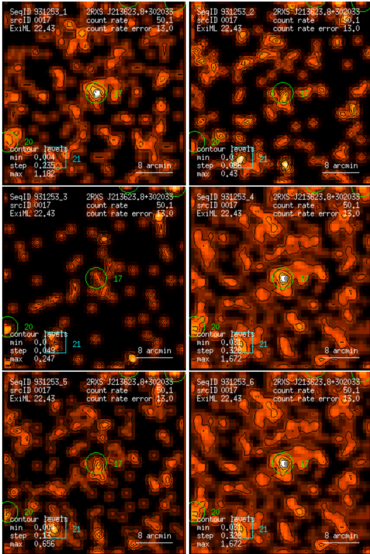
Figure 17: RASS 931253: detection 0017: band rate images, Gaussian filter: (1) PSPC channels 11 – 41, (2) 52 – 90, (3) 91 – 201, (4) 11 – 235, (5) 52 – 201, (6) 11 – 201. Broad band rates in counts/ks. Band rate contour levels in counts/ks/arcmin 2 .
