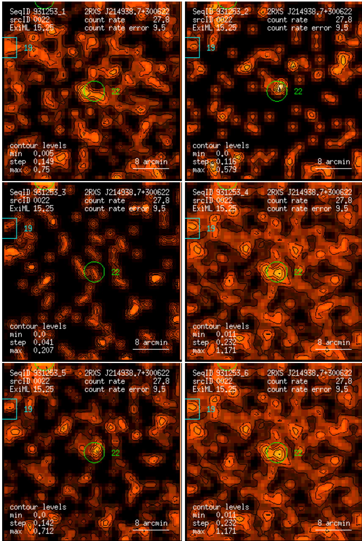
Figure 22: RASS 931253: detection 0022: band rate images, Gaussian filter: (1) PSPC channels 11 – 41, (2) 52 – 90, (3) 91 – 201, (4) 11 – 235, (5) 52 – 201, (6) 11 – 201. Broad band rates in counts/ks. Band rate contour levels in counts/ks/arcmin 2 .
