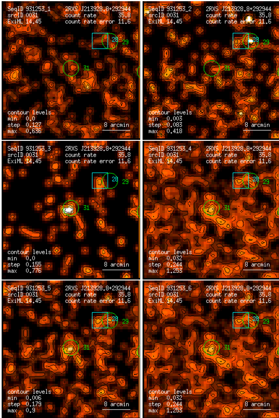
Figure 31: RASS 931253: detection 0031: band rate images, Gaussian filter: (1) PSPC channels 11 – 41, (2) 52 – 90, (3) 91 – 201, (4) 11 – 235, (5) 52 – 201, (6) 11 – 201. Broad band rates in counts/ks. Band rate contour levels in counts/ks/arcmin 2 .
