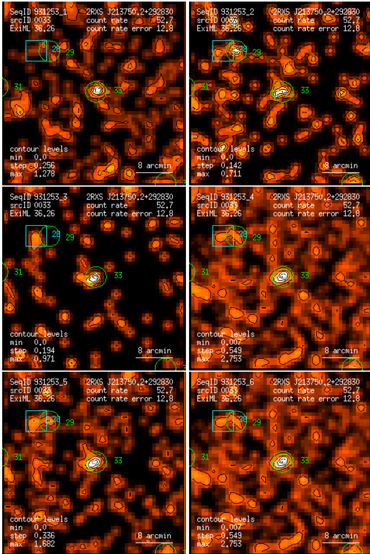
Figure 33: RASS 931253: detection 0033: band rate images, Gaussian filter: (1) PSPC channels 11 – 41, (2) 52 – 90, (3) 91 – 201, (4) 11 – 235, (5) 52 – 201, (6) 11 – 201. Broad band rates in counts/ks. Band rate contour levels in counts/ks/arcmin 2 .
