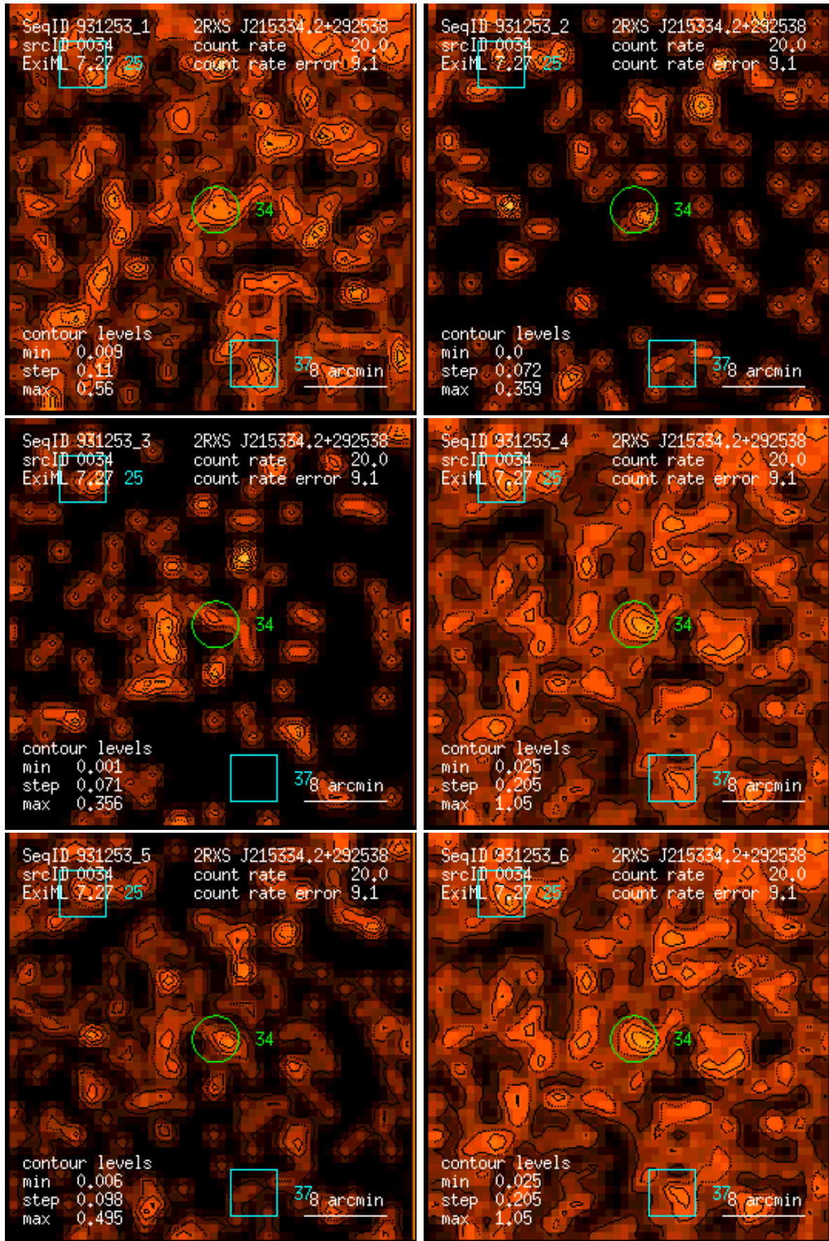
Figure 34: RASS 931253: detection 0034: band rate images, Gaussian filter: (1) PSPC channels 11 – 41, (2) 52 – 90, (3) 91 – 201, (4) 11 – 235, (5) 52 – 201, (6) 11 – 201. Broad band rates in counts/ks. Band rate contour levels in counts/ks/arcmin 2 .
