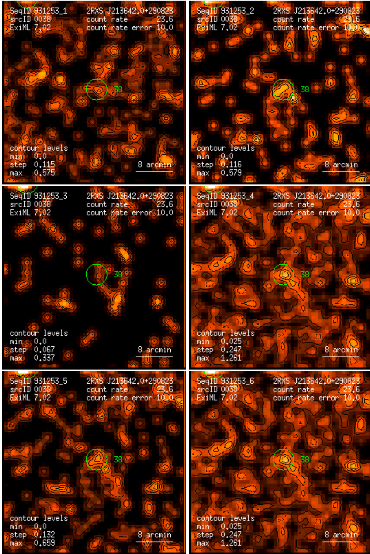
Figure 38: RASS 931253: detection 0038: band rate images, Gaussian filter: (1) PSPC channels 11 – 41, (2) 52 – 90, (3) 91 – 201, (4) 11 – 235, (5) 52 – 201, (6) 11 – 201. Broad band rates in counts/ks. Band rate contour levels in counts/ks/arcmin 2 .
