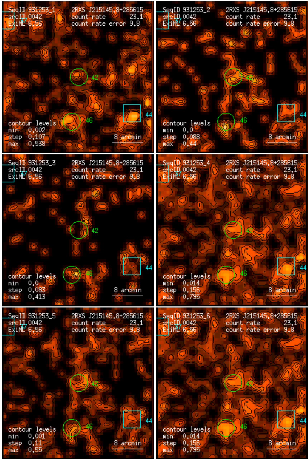
Figure 42: RASS 931253: detection 0042: band rate images, Gaussian filter: (1) PSPC channels 11 – 41, (2) 52 – 90, (3) 91 – 201, (4) 11 – 235, (5) 52 – 201, (6) 11 – 201. Broad band rates in counts/ks. Band rate contour levels in counts/ks/arcmin 2 .
