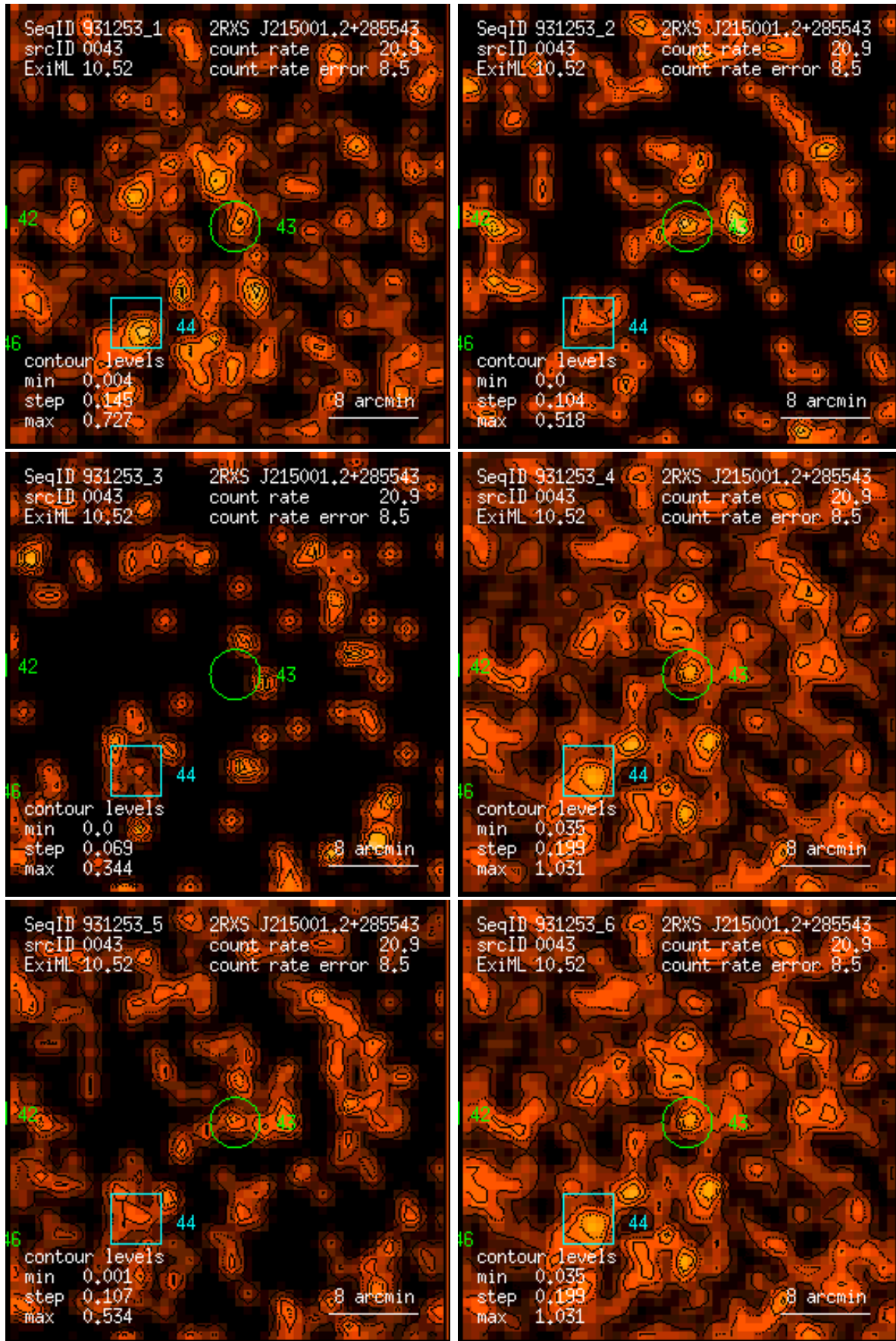
Figure 43: RASS 931253: detection 0043: band rate images, Gaussian filter: (1) PSPC channels 11 – 41, (2) 52 – 90, (3) 91 – 201, (4) 11 – 235, (5) 52 – 201, (6) 11 – 201. Broad band rates in counts/ks. Band rate contour levels in counts/ks/arcmin 2 .
