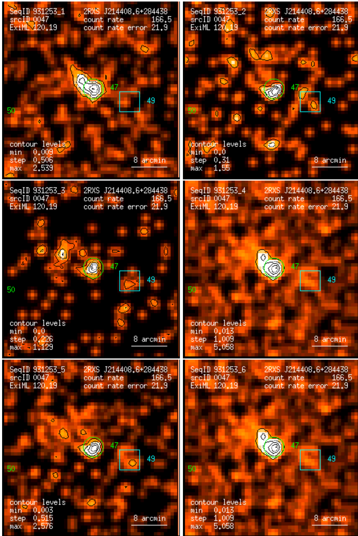
Figure 47: RASS 931253: detection 0047: band rate images, Gaussian filter: (1) PSPC channels 11 – 41, (2) 52 – 90, (3) 91 – 201, (4) 11 – 235, (5) 52 – 201, (6) 11 – 201. Broad band rates in counts/ks. Band rate contour levels in counts/ks/arcmin 2 .
