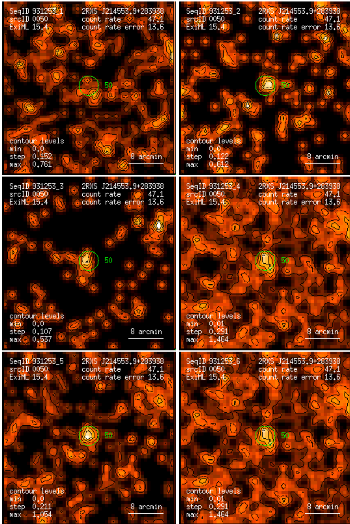
Figure 50: RASS 931253: detection 0050: band rate images, Gaussian filter: (1) PSPC channels 11 – 41, (2) 52 – 90, (3) 91 – 201, (4) 11 – 235, (5) 52 – 201, (6) 11 – 201. Broad band rates in counts/ks. Band rate contour levels in counts/ks/arcmin 2 .
