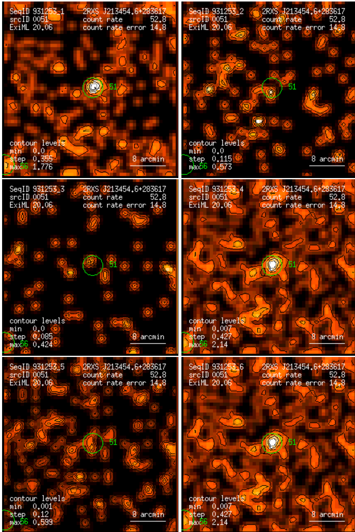
Figure 51: RASS 931253: detection 0051: band rate images, Gaussian filter: (1) PSPC channels 11 – 41, (2) 52 – 90, (3) 91 – 201, (4) 11 – 235, (5) 52 – 201, (6) 11 – 201. Broad band rates in counts/ks. Band rate contour levels in counts/ks/arcmin 2 .
