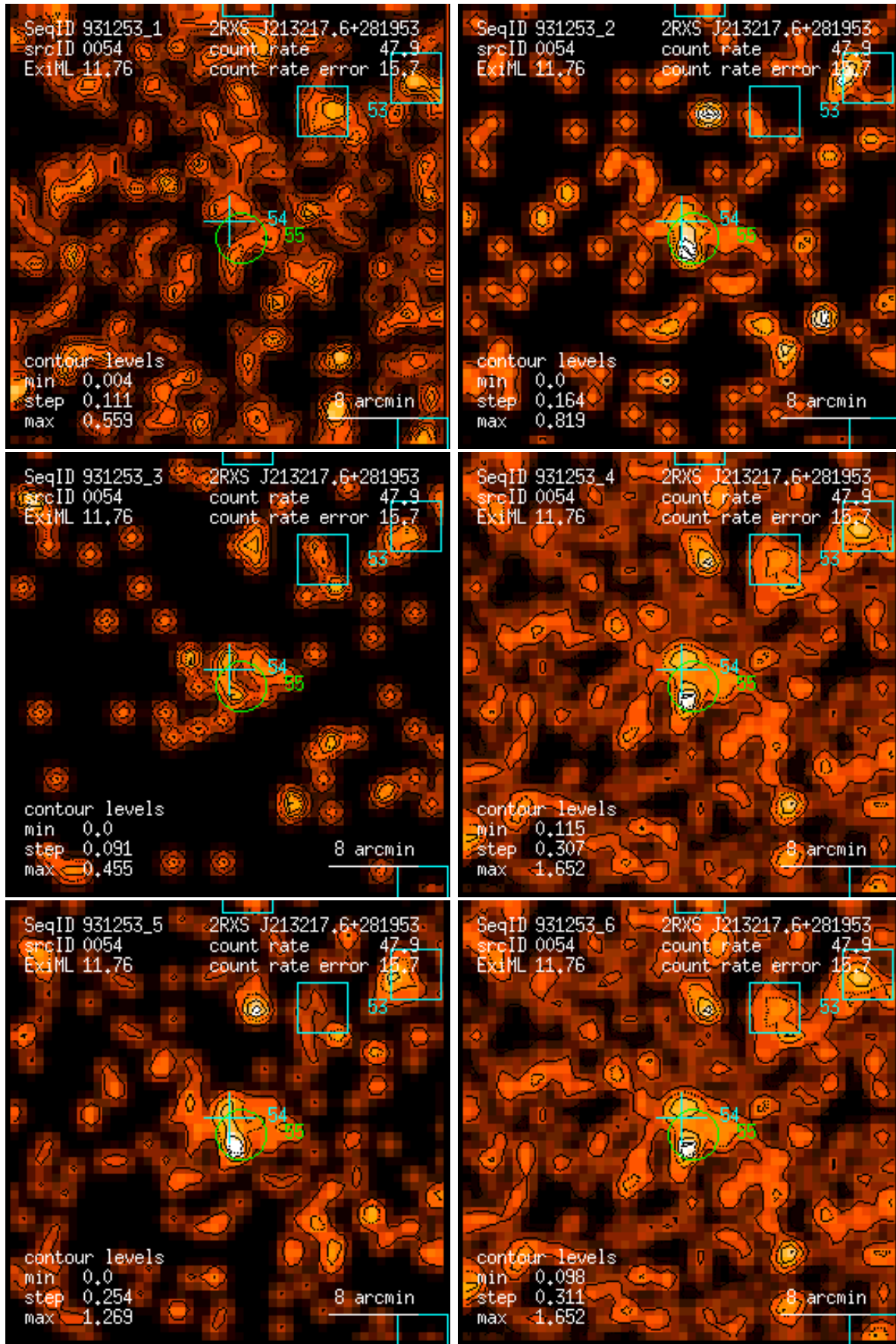
Figure 54: RASS 931253: detection 0054: band rate images, Gaussian filter: (1) PSPC channels 11 – 41, (2) 52 – 90, (3) 91 – 201, (4) 11 – 235, (5) 52 – 201, (6) 11 – 201. Broad band rates in counts/ks. Band rate contour levels in counts/ks/arcmin 2 .
