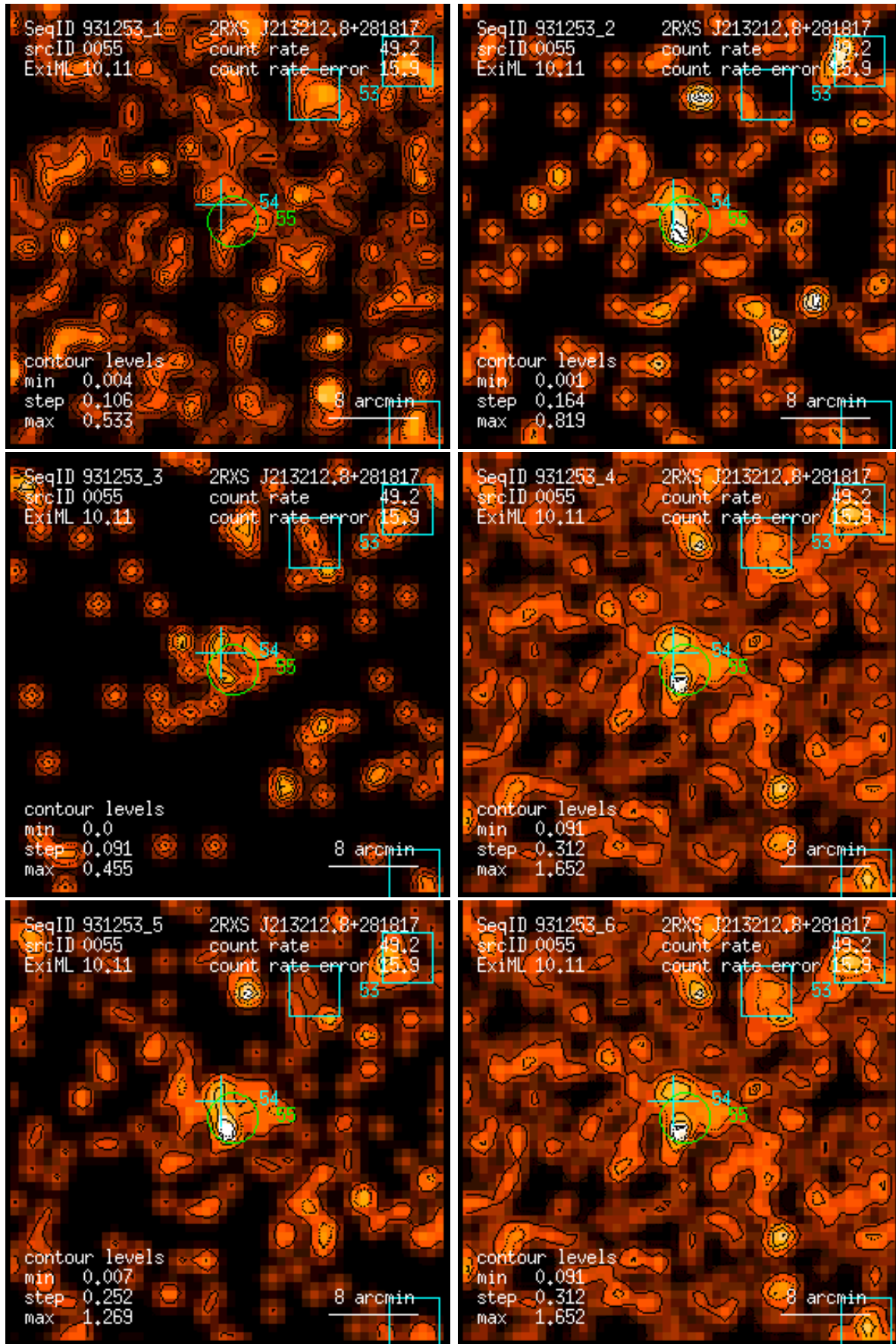
Figure 55: RASS 931253: detection 0055: band rate images, Gaussian filter: (1) PSPC channels 11 – 41, (2) 52 – 90, (3) 91 – 201, (4) 11 – 235, (5) 52 – 201, (6) 11 – 201. Broad band rates in counts/ks. Band rate contour levels in counts/ks/arcmin 2 .
