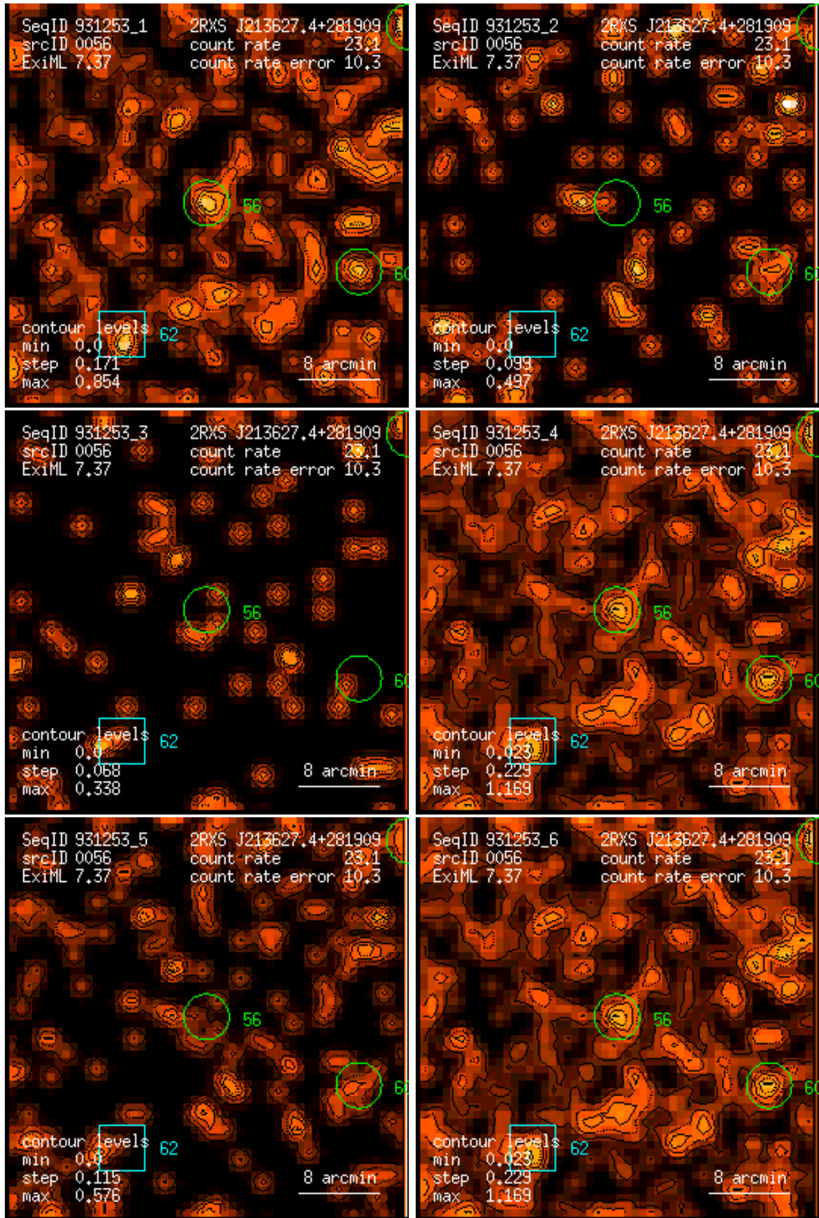
Figure 56: RASS 931253: detection 0056: band rate images, Gaussian filter: (1) PSPC channels 11 – 41, (2) 52 – 90, (3) 91 – 201, (4) 11 – 235, (5) 52 – 201, (6) 11 – 201. Broad band rates in counts/ks. Band rate contour levels in counts/ks/arcmin 2 .
