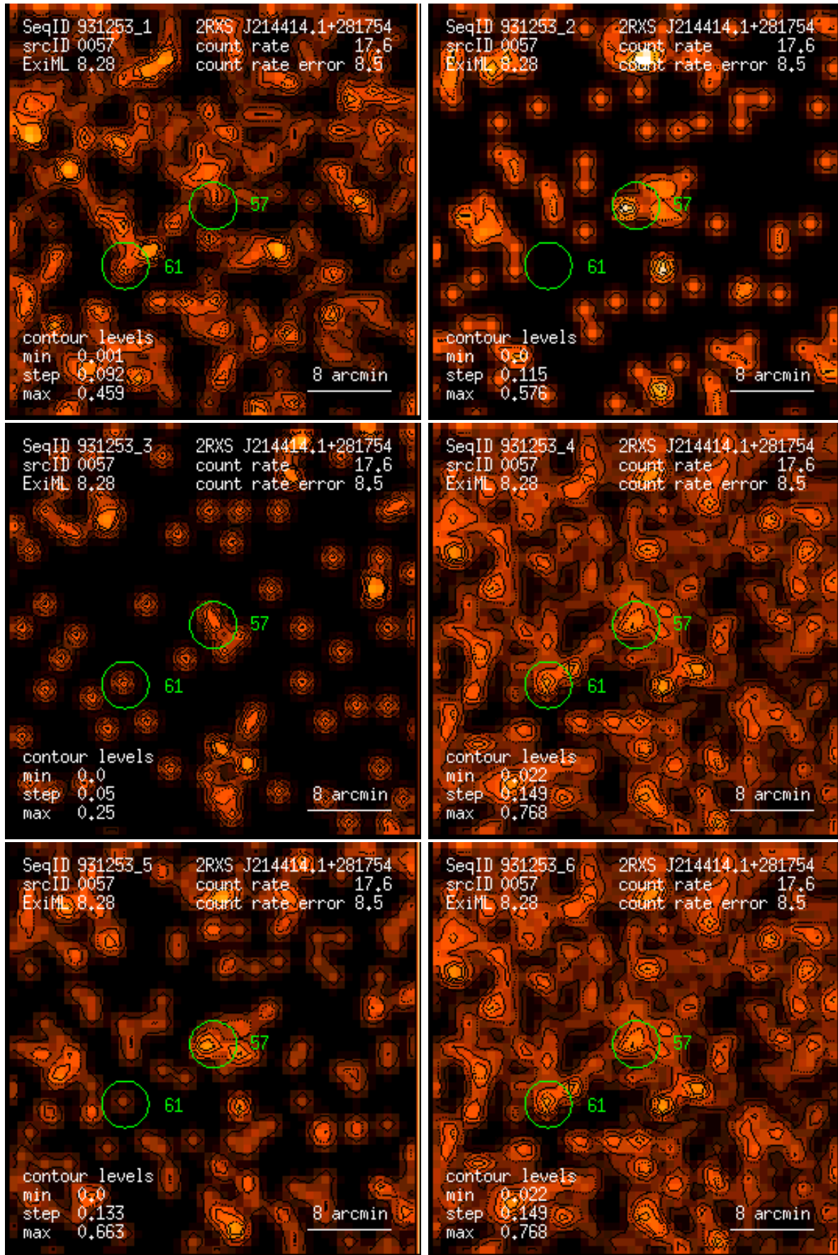
Figure 57: RASS 931253: detection 0057: band rate images, Gaussian filter: (1) PSPC channels 11 – 41, (2) 52 – 90, (3) 91 – 201, (4) 11 – 235, (5) 52 – 201, (6) 11 – 201. Broad band rates in counts/ks. Band rate contour levels in counts/ks/arcmin 2 .
