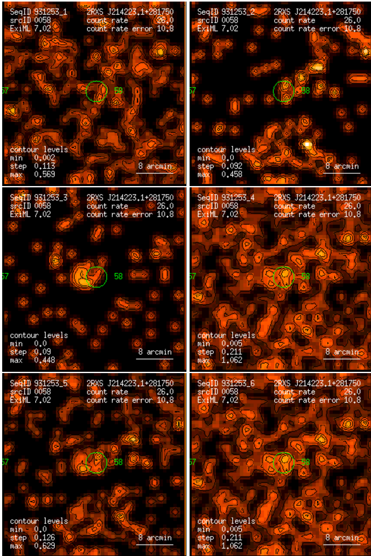
Figure 58: RASS 931253: detection 0058: band rate images, Gaussian filter: (1) PSPC channels 11 – 41, (2) 52 – 90, (3) 91 – 201, (4) 11 – 235, (5) 52 – 201, (6) 11 – 201. Broad band rates in counts/ks. Band rate contour levels in counts/ks/arcmin 2 .
